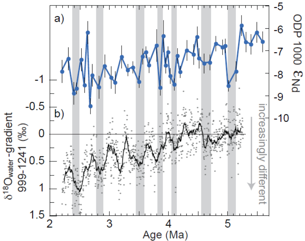
Figure 6a) Uncleaned planktonic foraminifera \epsilon_{Nd} for Site 1000. b) Difference in salinity between the Caribbean and the eastern equatorial Pacific, line is the 25-point running average [Groeneveld, 2005]. Gray bars indicate episodes of less radiogenic \epsilon_{Nd} in the Site 1000 record that correspond to maxima in the salinity-difference record.
