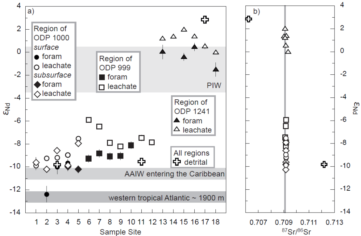
Figure 2a) \epsilon_{Nd} values for core top uncleaned planktonic foraminifera (filled symbols) and leachates (open symbols) and the detrital fraction (open crosses) in the region of ODP Sites 1000, 999 and 1241. Numbers on the x-axis refer to Sites in Table S1 and Figure S1. 2\sigma errors are indicated by the gray bars but in most cases are smaller than symbol size. Horizontal shading indicates \epsilon_{Nd} signatures of water masses: PIW [Piepgras and Wasserburg, 1982; Piepgras and Jacobsen, 1988], AAIW entering the Caribbean, and western tropical Atlantic ~1900 m [Piepgras and Wasserburg, 1987; Huang et al. , 2014]. b) ^{87}Sr/^{86}Sr vs \epsilon_{Nd} for core-top leachate and detrital samples. Symbols as before. The composition of modern seawater Sr [McArthur et al. , 2001] is indicated by the vertical line.
