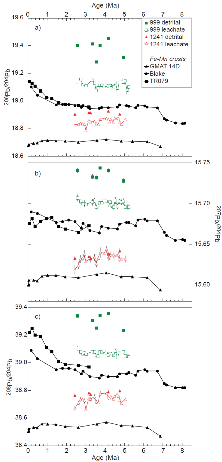
Figure 4a) ^{206}\text{Pb}/^{204}\text{Pb} ; b) ^{207}\text{Pb}/^{204}\text{Pb} ; and c) ^{208}\text{Pb}/^{204}\text{Pb} values for Sites 999 and 1241. 2\sigma errors are indicated by the gray bars but in many cases are smaller than symbol size. Also shown are Fe-Mn crust data from GMAT 14D [Frank et al. , 1999], Blake [Reynolds et al. , 1999] and TR079 [Reynolds et al. , 1999]. Symbols are the same for all plots.
