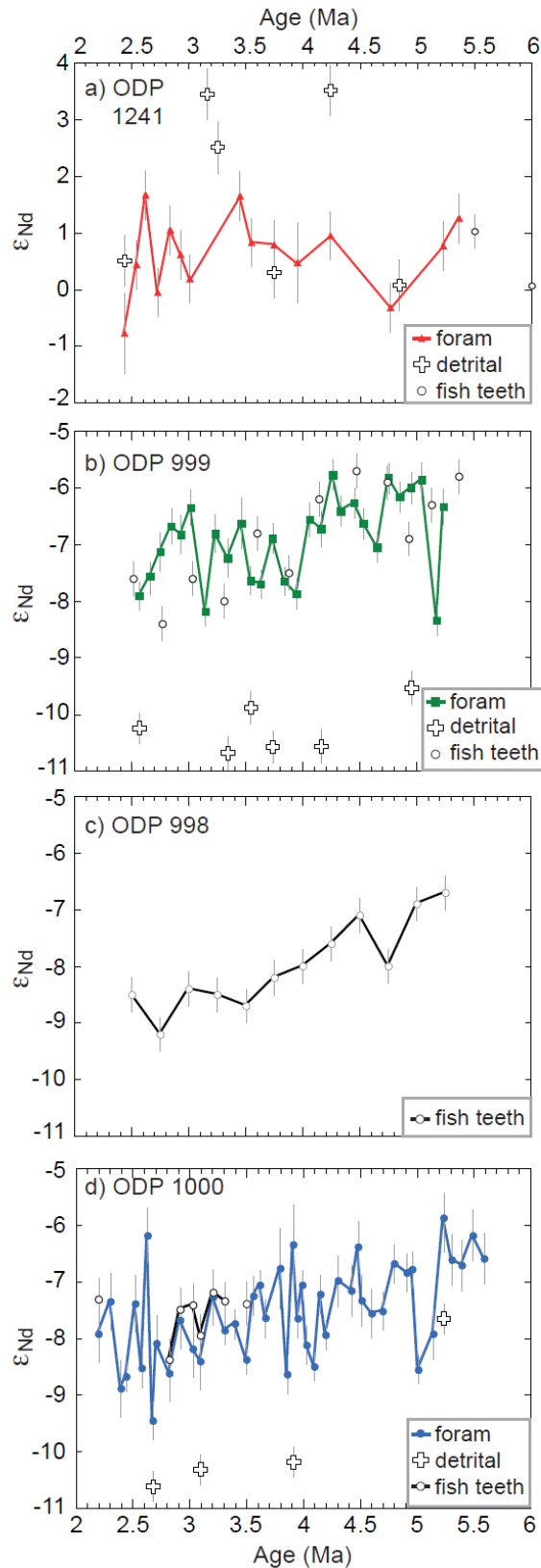
Figure 3 \epsilon_{Nd} composition of uncleaned planktonic foraminifera (foram), detrital fraction and fish teeth. Fish teeth data for ODP Site 1241 from Newkirk and Martin [2009]. 2\sigma errors are indicated by the gray bars.
