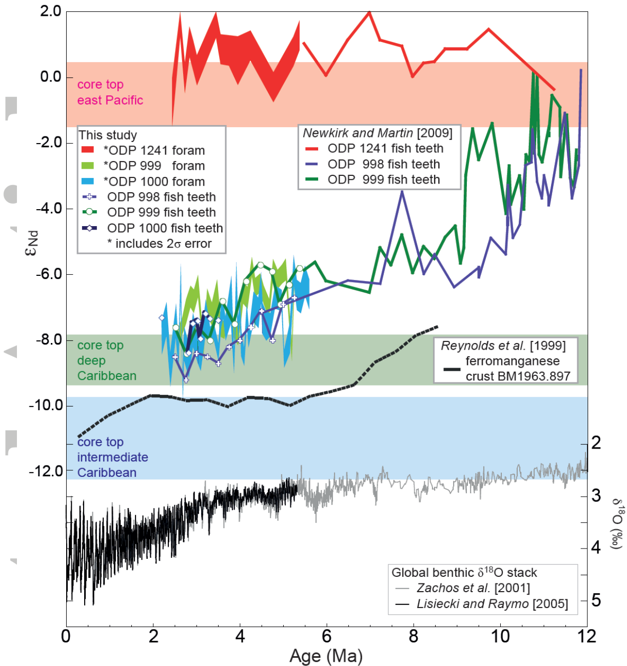
Figure 5 Compilation of \epsilon_{Nd} data for ODP Sites 1241, 998, 999 and 1000 from this study and Newkirk and Martin [2009]. Colored horizontal bars indicate the core top foraminifera \epsilon_{Nd} results. Also shown is the \epsilon_{Nd} of ferromanganese crust BM1963.897, taken from ~850m water depth on the Blake Plateau [Reynolds et al., 1999] and the global benthic \delta^{18}O stack of Zachos et al. [2001] and Lisiecki and Raymo [2005].
