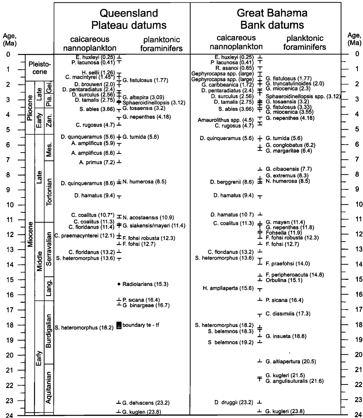
Figure 4. Age models used at the Queensland Plateau and at Great Bahama Bank. Age of datums are converted to the Berggren et al. [1995] timescale. Asterisks indicate datums not discussed in Berggren et al. [1995]. These ages are after Gartner et al. [1993a]. Boundary te-tf refers to East Indian Letter Stage Classification of large benthic foraminifers. See text for further discussion
