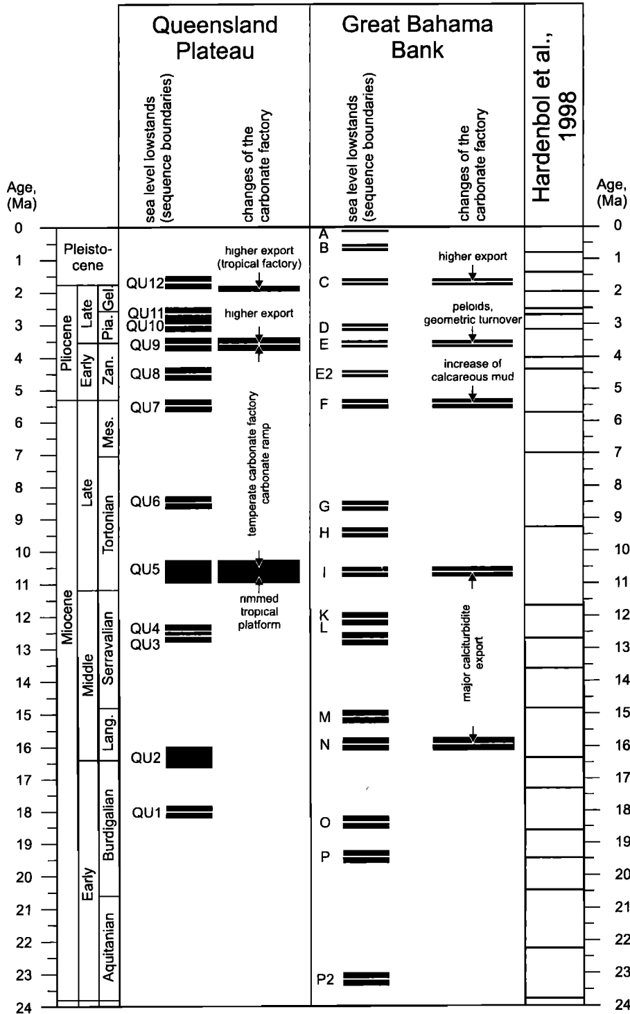
Figure 3. Neogene sequence boundaries of the Queensland Plateau and Great Bahama Bank and major changes in shallow-water carbonate production. Timescale is after Berggren et al. [1995]. Sequence boundaries A-P2 are after Eberli et al. [1997], and E2 is after Betzler et al. [1999]. Black boxes indicate age uncertainties.
