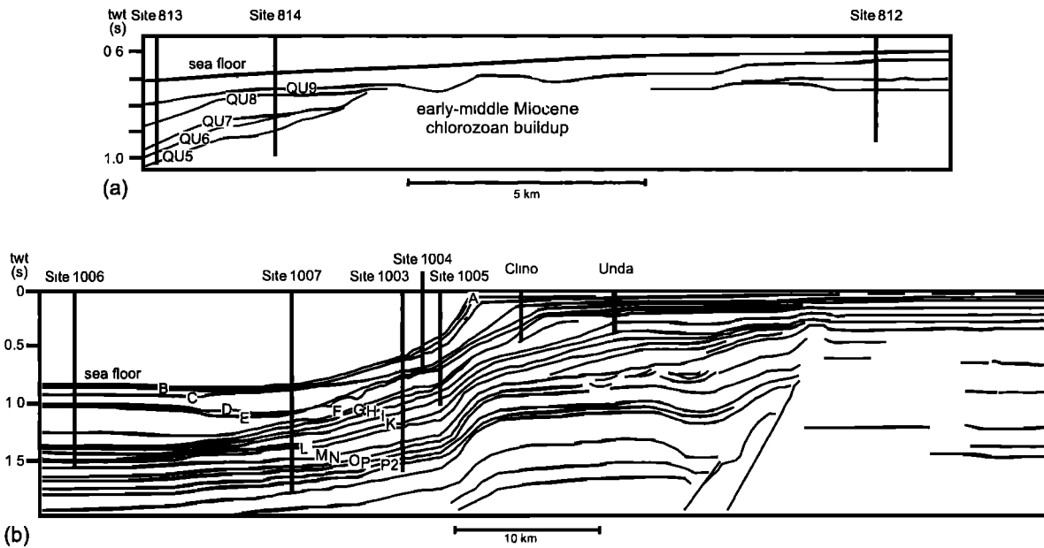
Figure 2. Carbonate platform geometry in one of the seismic lines at the southern part of the Queensland Plateau (a) showing late Miocene–early Pliocene sequence boundaries [modified after Betzler, 1997 ] and (b) sequence boundaries at Great Bahama Bank [modified after Eberli et al., 1997 ]
