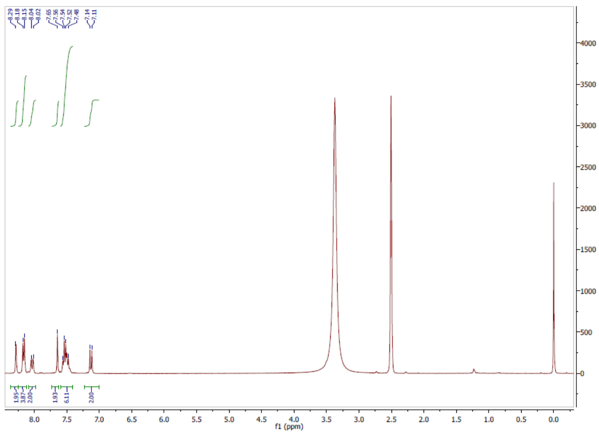
Figure S9. ^1\text{H} NMR of 4,4'-(5,5-difluoro-1,9-diphenyl-5H-4 \lambda 4 ,5 \lambda 4 -dipyrrolo[1,2- c :2',1'- f ][1,3,5,2]triazaborinine-3,7-diyl)bis(2-chlorophenol) (di-Cl-di-OH-complex).
