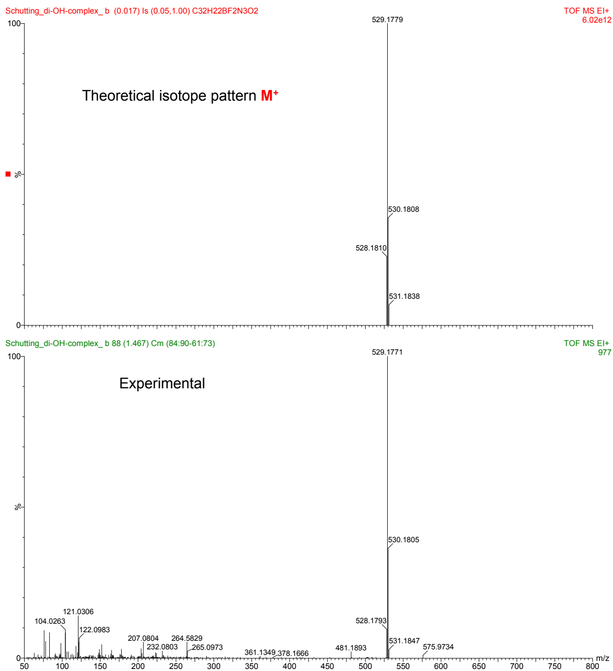
Figure S4. EI-DI Mass spectrum of 4,4'-(5,5-difluoro-1,9-diphenyl-5 H -4 \lambda 4 ,5 \lambda 4 -dipyrrolo[1,2- c :2',1'- f ][1,3,5,2]triazaborinine-3,7-diyl)diphenol (di-OH-complex).
