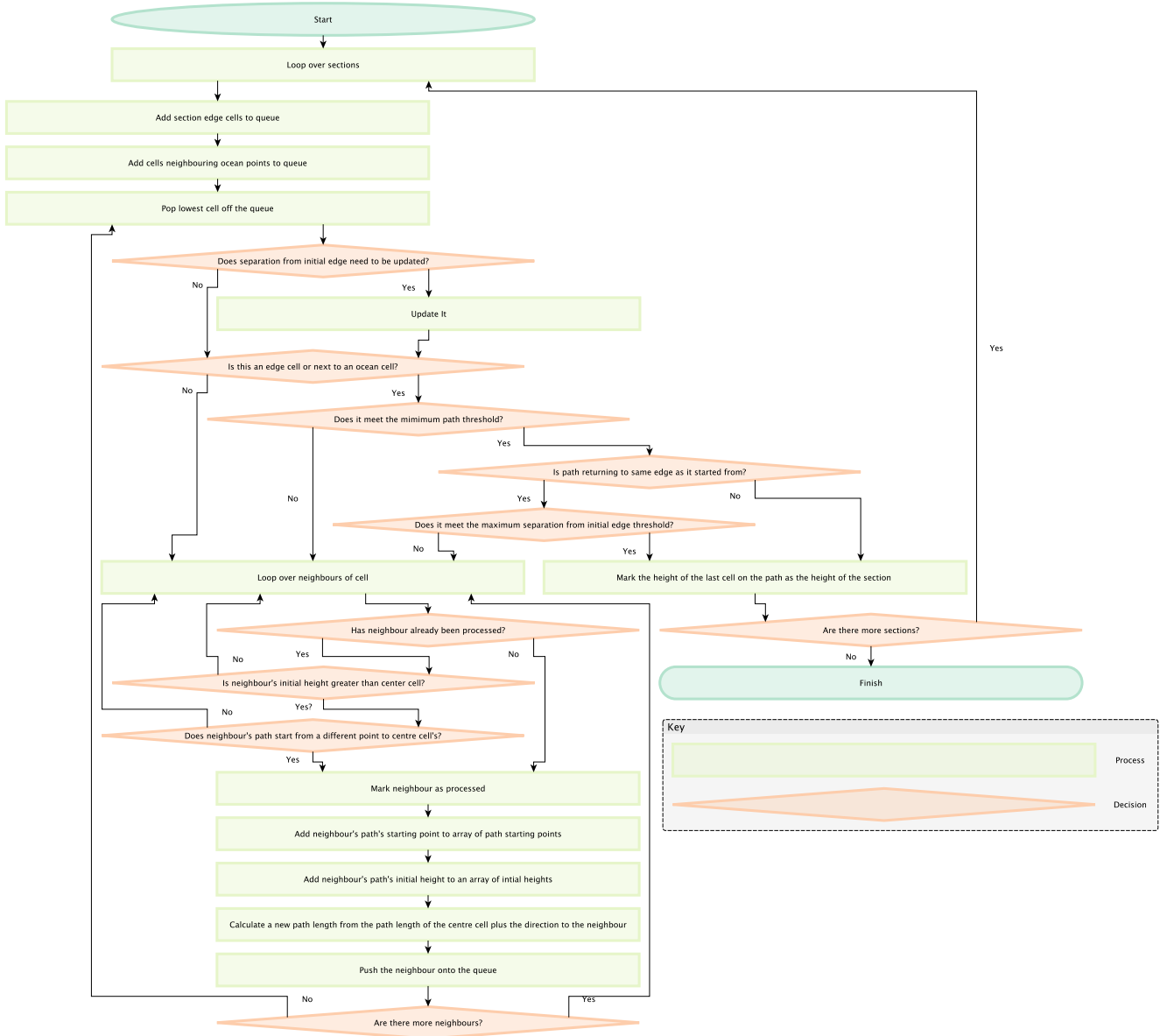
Figure S1. Flow diagram illustrating the steps of the orography upscaling algorithm.
