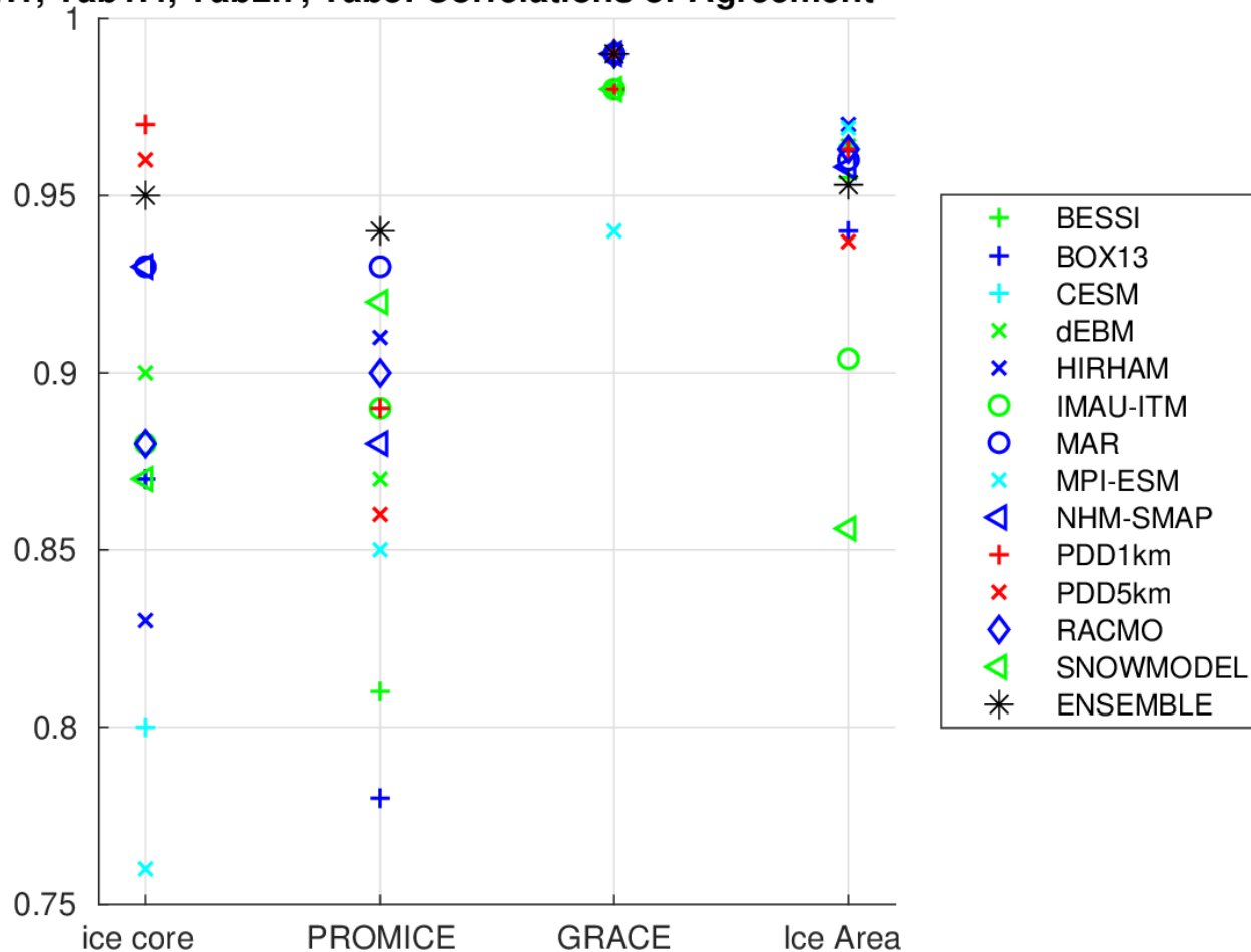
Tab1.1, Tab1.4, Tab2.7, Tab3: Correlations or Agreement
