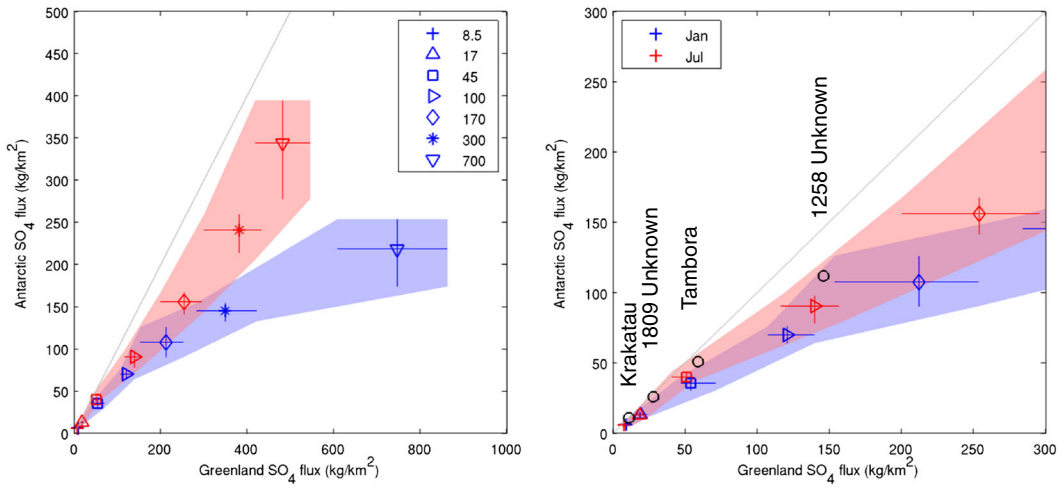
Figure 7. Bias-corrected modeled Antarctic versus Greenland mean volcanic sulfate deposition for varying stratospheric \text{SO}_2 injection magnitudes. Modeled deposition flux values are scaled by a factor of 1/4.7 based on comparisons of modeled versus ice core-derived deposition flux for Pinatubo (see Figure 2). Ensemble mean deposition fluxes shown by symbols, with ensemble variability indicated by horizontal and vertical lines. Shading indicates expected variability range and is produced by linearly interpolating between the envelopes of the variability range of each experiment. Right-hand panel shows zoom-in of left-hand panel, with Antarctic and Greenland average ice core sulfate flux estimates from GOR07 shown by black circles for four tropical eruptions with unambiguous signals in both Greenland and Antarctic ice cores.
