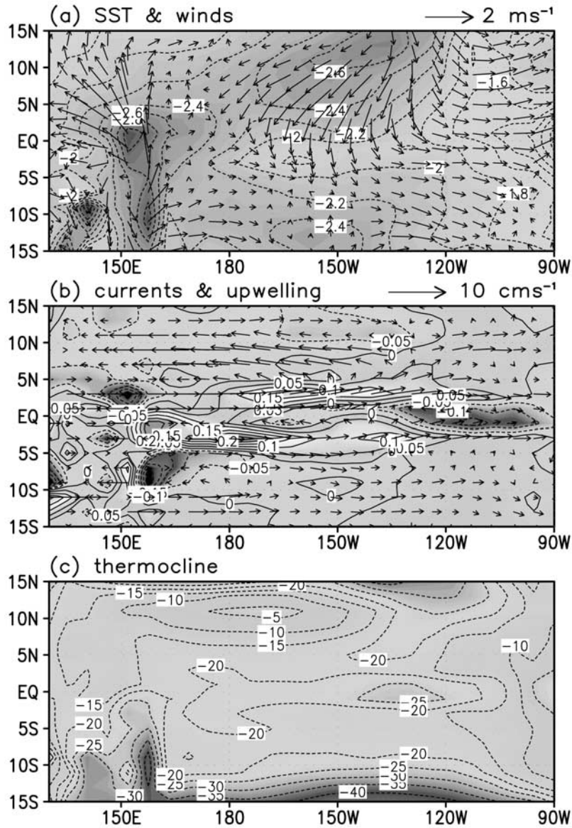
Figure 2. Simulated difference of SST (K), wind (m/s), surface current (cm/s), upwelling (10 -3 cm/s) and thermocline depth (m) between CSM LGM and present-day simulation. Data are interpolated onto the grid of our intermediate tropical model. See color version of this figure at back of this issue.
