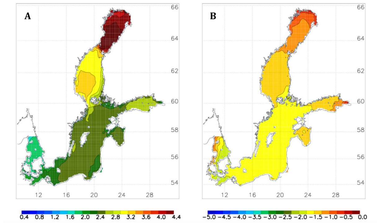
Figure 2: Changes in A) summer mean SST (°C) and B) annual mean SSS in the Baltic Sea (g kg -1 ) between the years 2069-2098, calculated using the ensemble mean variation of regional climate models (adapted from Meier et al., 2012).
