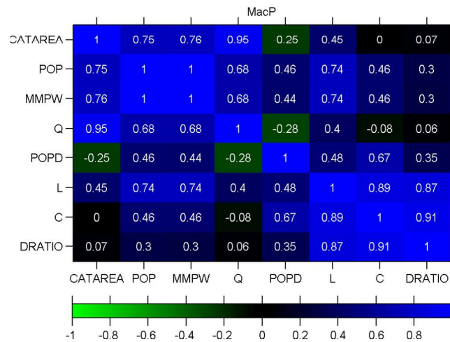
Figure S2: Matrix of Pearson correlation coefficients for microplastic (top panel) and macroplastic (lower panel) between catchment attributes and plastic concentration and loads. Variables: catchment area (CATAREA), total population in the catchment (POP), the Mismanaged plastic waste generation in the catchment (MMPW), mean river discharge (Q), population density (POPD), observed plastic load (L), plastic mass concentration (C), plastic delivery ratio (DRATIO)
