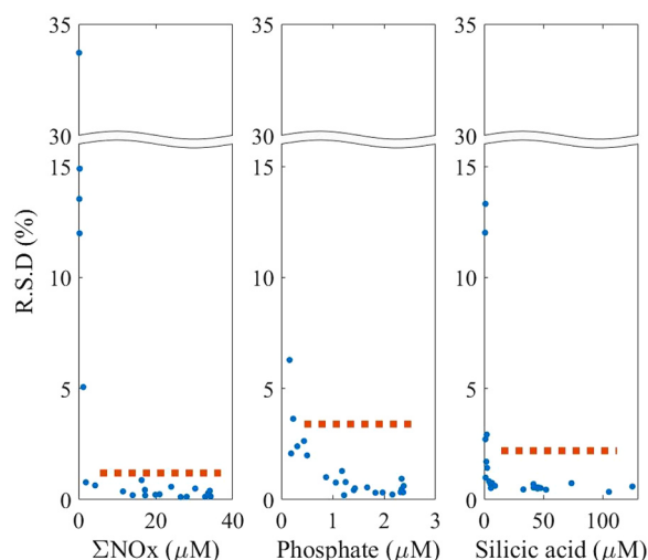
Fig. 2. The mean concentration and relative standard deviation (R.S.D.) calculated from the analysis of 10 samples collected from the same Niskin water sampler (blue symbols). This approach incorporates uncertainties associated with sampling and short term analytical reproducibility. One data point with a mean phosphate concentration of 0.01 \mu\text{M} was removed as it was deemed to be below the limit of detection. The dashed orange line denotes the combined uncertainty estimate calculated in this study ( k = 1 ). This approach incorporates uncertainties associated within laboratory reproducibility and systematic bias. (For interpretation of the references to color in this figure legend, the reader is referred to the web version of this article).
