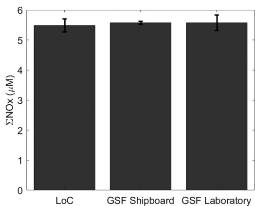
Fig. 3. The mean \Sigma\text{NOx} concentration ( \pm 1 S.D.) for CRM KANSO-CD determined using gas segmented flow analysis (GSF) and Lab-on-Chip analysers (LoC). The certified value is 5.63 \pm 0.05 \mu\text{M} .
