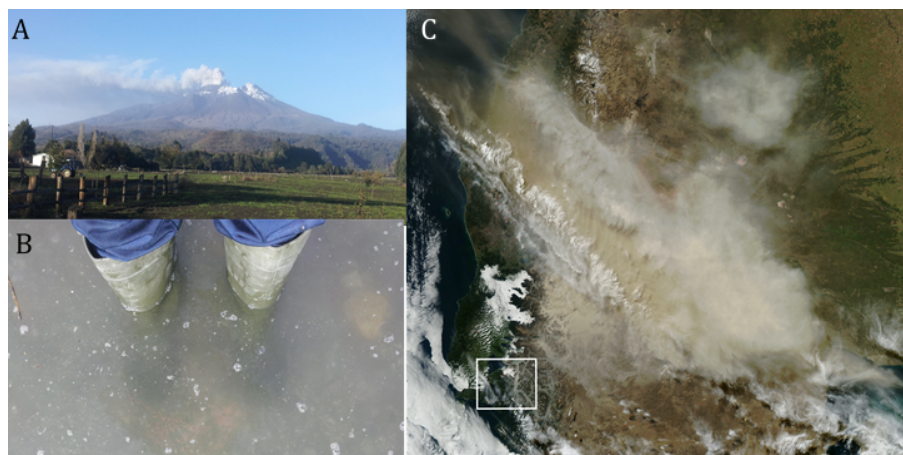
Figure 2. (a) Calbuco volcano ash plume 6 May 2015. (b) Reloncaví Fjord water with atypical high turbidity due to the ash loading, Cochamó town 6 May. (c) Ash cloud visible on MODIS Aqua satellite from the NASA Earth Observatory, 23 April ( http://earthobservatory.nasa.gov/NaturalHazards/view.php?id=85767&eocon=home&eoeci=nh , last access: 1 February 2021). The highlighted box in panel (c) corresponds to Fig. 1c.
