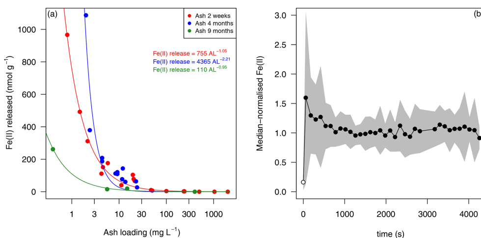
Figure 7. Fe(II) release from Calbuco ash into seawater. (a) Mean Fe(II) released into South Atlantic seawater over a 30 min leach at 5–7 °C. The same batch of Calbuco ash was subsampled and used to conduct experiments on three occasions after the 2015 eruption (2 weeks, 4 months and 9 months since ash collection). The lines are power law fits, with the associated equations shown in the legend. (b) The three time series of Fe(II) concentrations following ash addition are considered collectively by normalising the measured concentrations, such that 1.0 represents the median Fe(II) concentration measured in each experiment. All experiments were conducted for at least 30 min, those conducted with 4- and 9-month-old ash were extended for 1 h. The black line shows the mean response over 34 leach experiments with varying ash loading, and the shaded area shows \pm 1 standard deviation. The initial Fe(II) concentration (pre-ash addition at 0 s) in all cases was below detection; thus, the detection limit is plotted at 0 s (open circle). Source data are provided in the Supplement (Table S2).
