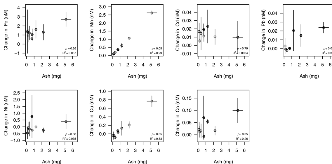
Figure 6. Change in trace metal concentrations after varying ash addition to 100 mL of South Atlantic seawater for a 10 min leach duration at room temperature. Initial (mean \pm standard deviation) dissolved trace metal concentrations – deducted from the final concentrations to calculate the change as a result of ash addition – were 0.98 \pm 0.03 nM Fe, 0.38 \pm 0.04 nM Cd, 13 \pm 2 pM Pb, 6.58 \pm 0.76 nM Ni, 0.84 \pm 0.07 nM Cu, 145 \pm 9 pM Co and 0.72 \pm 0.05 nM Mn. Error bars are standard deviations from triplicate treatments with similar ash loadings. p values and R^2 values for a linear regression are annotated. Source data are provided in the Supplement (Table S5). The same data with individual replicates are also shown in the Supplement (Fig. S1).
