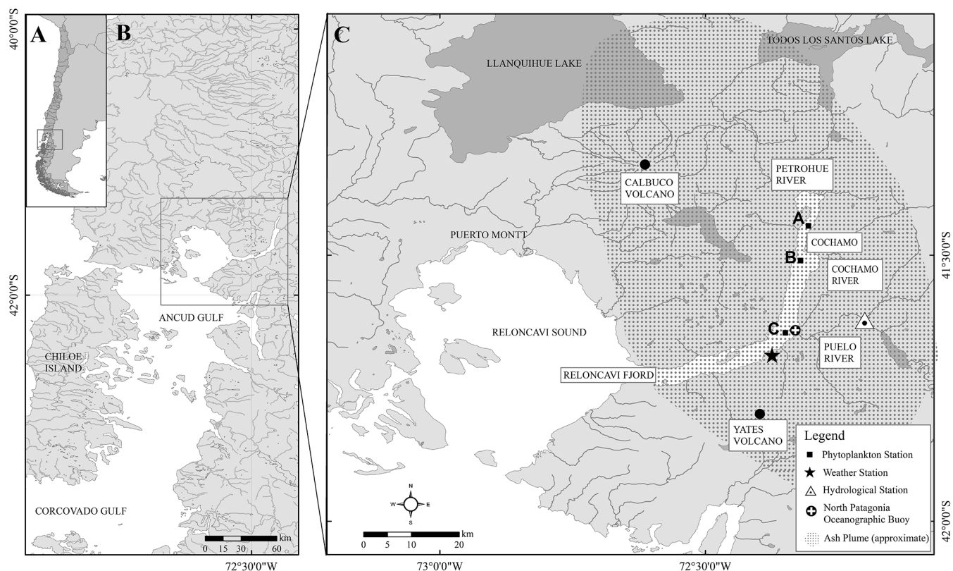
Figure 1. The Calbuco region showing the location of Reloncaví Fjord, three major rivers (the Petrohué, Cochamó and Puelo) discharging into the fjord, the three stations (black squares; panel c) used to assess changes in phytoplankton abundance following the eruption, a hydrological station that monitors the Puelo River flow, a weather station and the location of a long-term mooring within the fjord. The approximate extent of the ash plume in the week following the first eruption is illustrated, as estimated in technical reports issued by the Servicio Nacional de Geología y Minería (Chile).
