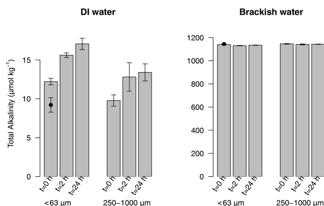
Figure 5. Total alkalinity released after leaching 4.5 \text{ g L}^{-1} of ash of two size fractions (< 63 and 250–1000 \mu\text{m} ) in deionised water (DI water) and brackish water. T_0 is “time zero” and was measured after 1 min of mixing; T_{2H} was measured after 2 h of mixing; T_{24H} was measured after 24 h of mixing. n = 4 for all treatments (mean \pm standard deviation plotted). The initial (pre-ash addition) alkalinity is marked by a black dot superimposed on the left T_0 . Source data are provided in the Supplement (Table S4).
