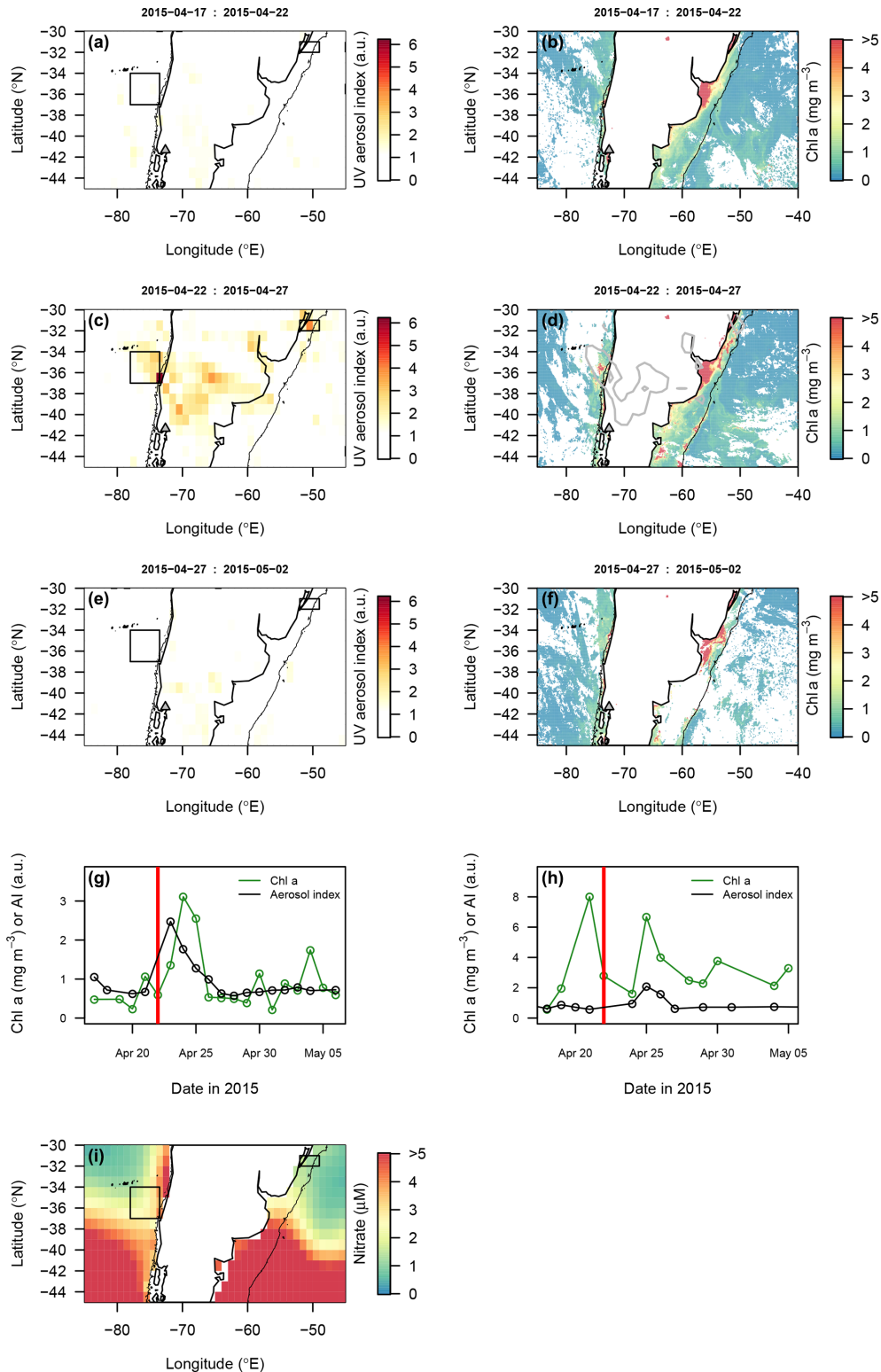
Figure 8. Potential biological impact of the 2015 Calbuco eruption observed via satellite remote sensing. (a–f) Spatial maps showing the distribution of ash in the atmosphere (UV aerosol index) and corresponding images of chlorophyll a . Images were composited over 5 d periods. Grey lines in the chlorophyll maps correspond to the UV aerosol index = 2 a.u. contour. (g, h) Time series of the UV aerosol index and chlorophyll a for regions of the Pacific (g) and Atlantic (h) oceans, identified by boxes in the maps. Red vertical lines (22 April) indicate the first eruption date. (i) Mean World Ocean Atlas surface \text{NO}_3 concentrations. Thin black lines indicate the 500 m bathymetric depth contour.
