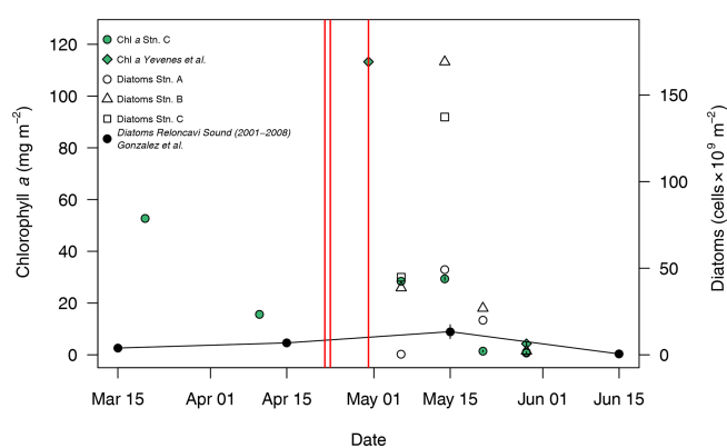
Figure 4. Changes in integrated (0–15 m) diatom abundance and chlorophyll a for Reloncaví Fjord in April–May 2015. Locations are as per Fig. 1; the eruption dates are marked with red lines. Historical diatom data from Reloncaví Sound (2001–2008, integrated to 10 m depth, mean \pm standard error, González et al., 2010) and additional chlorophyll data from 2015 (“Station 3” from Yevenes et al., 2019, approximately corresponding to station C herein) are also shown.
