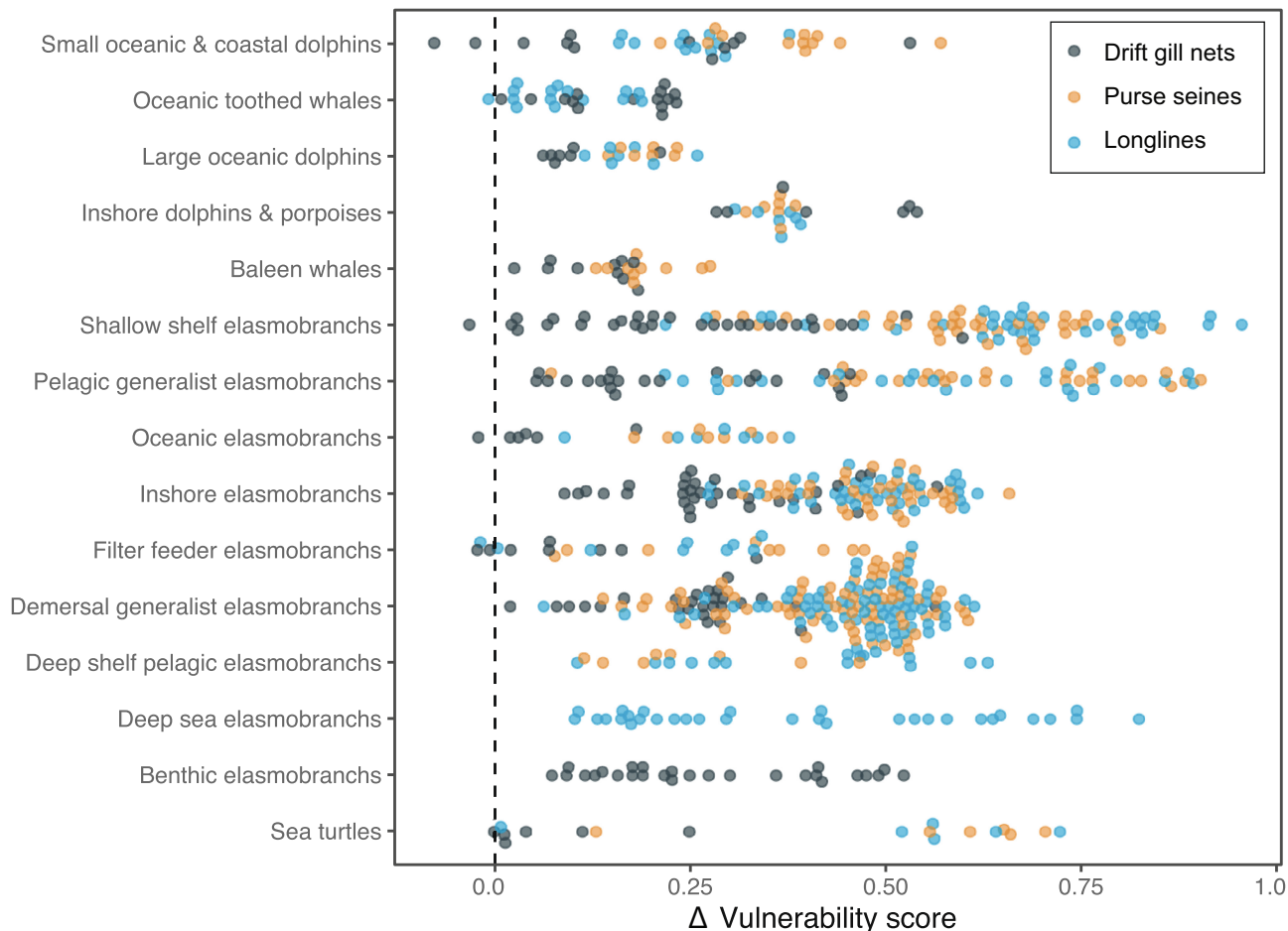
FIGURE 5 Differences in the vulnerability scores for 319 species in the three tuna gears using two different PSA methods. Most vulnerability scores were higher using the score-based PSA (delta vulnerability is positive)
