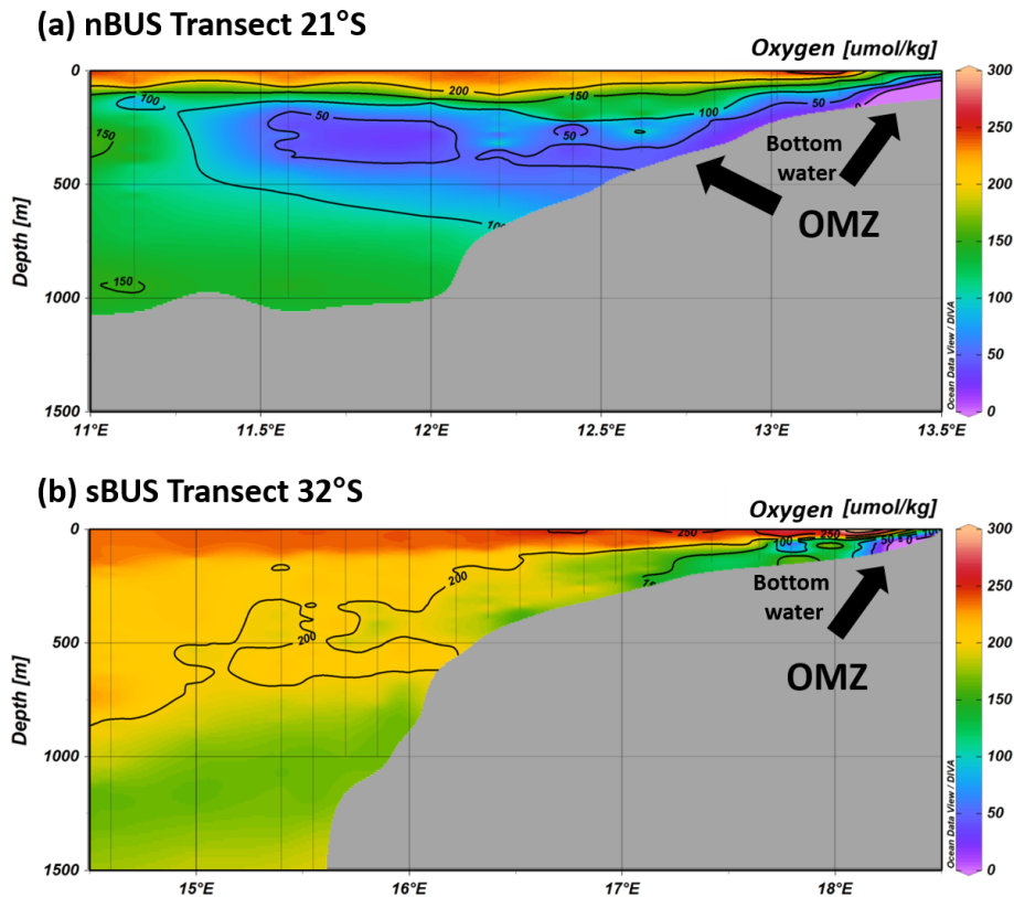
Figure 2. Oxygen concentrations along a transect in the nBUS and sBUS during cruise SO285, showing the near-bottom OMZ in the nBUS (a) and sBUS (b), as well as the OMZ on the continental slope in the nBUS. Oxygen data (Niko Lahajnar, unpublished data) are from CTD (conductivity, temperature, depth) casts conducted during cruise SO285. Graphic created with Ocean Data View, https://odv.awi.de (Schlitzer, 2024).
