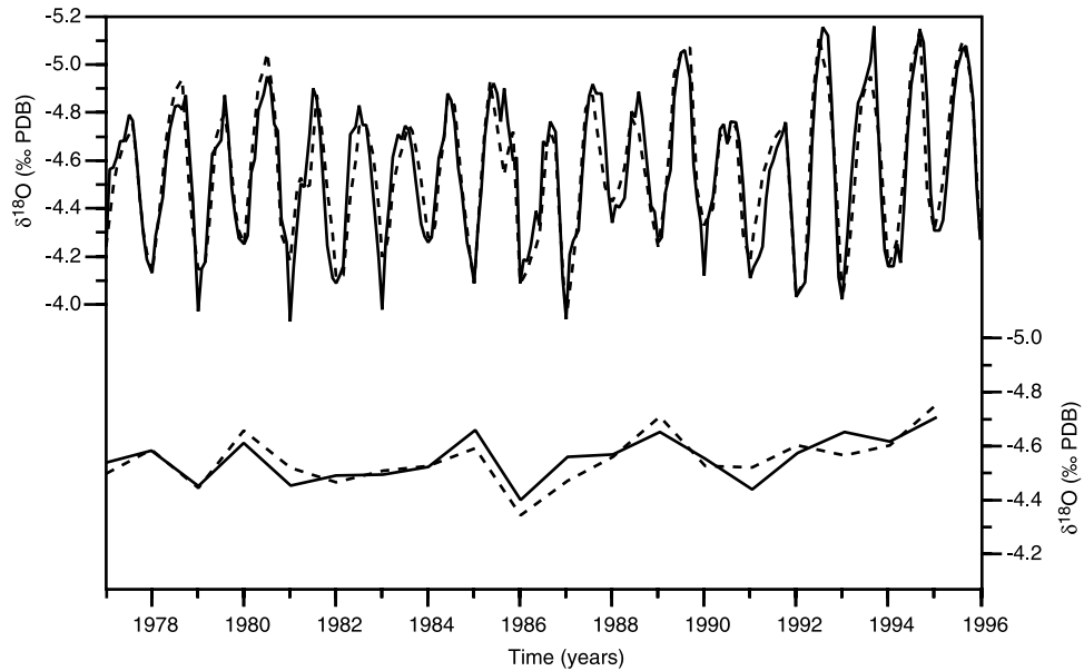
Figure 5. The upper curve shows the comparison of monthly and bimonthly resolved coral \delta^{18}\text{O} time series for the period 1977–1995. The lower curve shows the annual means computed from the monthly and bimonthly \delta^{18}\text{O} time series.
