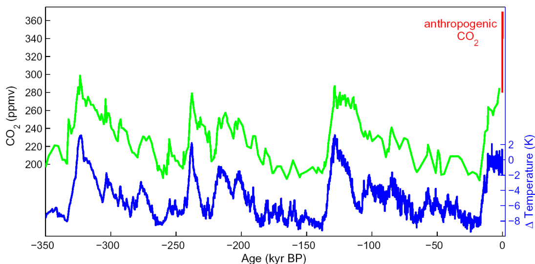
Figure 1. Records of CO 2 (green) and temperature (blue) over the past 350,000 years from the Vostok ice core, after [Petit et al., 1999]. Part of these data were used by [Lorius et al., 1990] to estimate climate sensitivity. The recent anthropogenic rise in CO 2 ([IPCC, 2001]) is marked in red.
