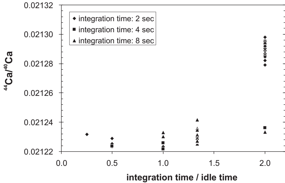
Figure 2.2: Set of measurements with different integration times and different integration to idle time ratios. The measurements with a 2 second integration time and 1 second idle time (integration time to idle time ratio = 2) show the highest ^{44}\text{Ca}/^{40}\text{Ca} ratios. However, increasing the idle time to 4 seconds results in lower ^{44}\text{Ca}/^{40}\text{Ca} ratios independent from the ratio of the integration time to idle time.
