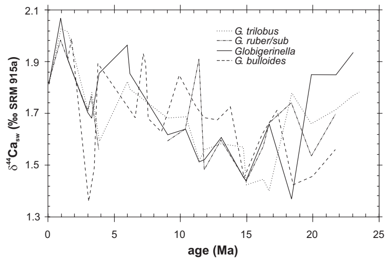
Figure 6.3: \delta^{44}\text{Ca}_{sw} records assuming a change of a between 1.5 and 3 Ma of G. ruber/subquadratus and Globigerinella spp. shifting \delta^{44}\text{Ca}_{sw} towards the G. trilobus -record. This leads to matching records of all four studied species.
