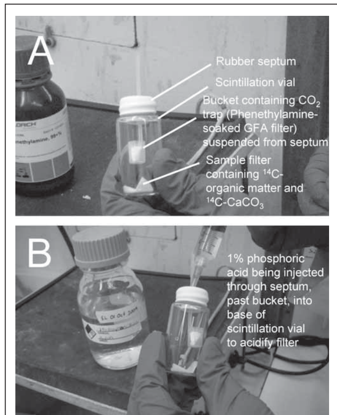
Figure 12.3 Sample manipulations involved in the microdiffusion technique for measuring phytoplankton calcification and primary productivity (Paasche & Brubak, 1994; Balch et al. , 2000). (A) Basic set-up showing scintillation vial with filter (which contains ^{14}\text{C} -labeled particulate organic matter and ^{14}\text{C} - \text{CaCO}_3 ) in the bottom. The vial is sealed with a rubber septum from which is suspended a plastic bucket containing a GFA filter soaked with 0.2 ml of phenethylamine (to act as a \text{CO}_2 trap). (B) Separation of ^{14}\text{C} -labeled POC and PIC begins when a syringe is used to inject 1.0 ml of 1% phosphoric acid, past the bucket/trap onto the filter in the bottom of the vial. The acid drives the ^{14}\text{C} - \text{CaCO}_3 into the head space as ^{14}\text{C} - \text{CO}_2 where it is subsequently trapped in the phenethylamine trap over the next 24 h. Following the diffusion process, the vial is opened and the bucket (containing activity originally associated with ^{14}\text{C} - \text{CaCO}_3 ) is placed in a separate vial with 1 ml distilled water plus 10 ml scintillation cocktail. The original vial with filter (containing ^{14}\text{C} -organic matter) and 1 ml acid has 10 ml of scintillation cocktail added. Both vials are then placed in a high sensitivity scintillation counter for measurement of their respective radioactivity.
