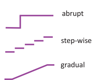
Figure 6.6 Possible time courses for \text{CO}_2 manipulation.
