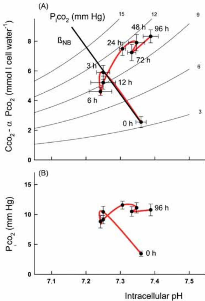
Figure 9.1 pH bicarbonate diagram (A) depicting the interrelated changes of intracellular acid-base variables pH (pH i ), bicarbonate and P i CO 2 (P i CO 2 ) over time and in relation to the non-bicarbonate buffer (β NB ) line. Initial changes in pH i are driven by the accumulation of CO 2 which leads to a rise in P i CO 2 (B), titrates non-bicarbonate buffers and is therefore paralleled by an accumulation of bicarbonate (A). Transmembrane ion exchange and metabolic processes interfere after 3 h and, after an initial base loss, lead to continued net bicarbonate accumulation while the respiratory acidosis persists with more or less constant P i CO 2 levels (based on data from Pörtner et al. , 1998).
