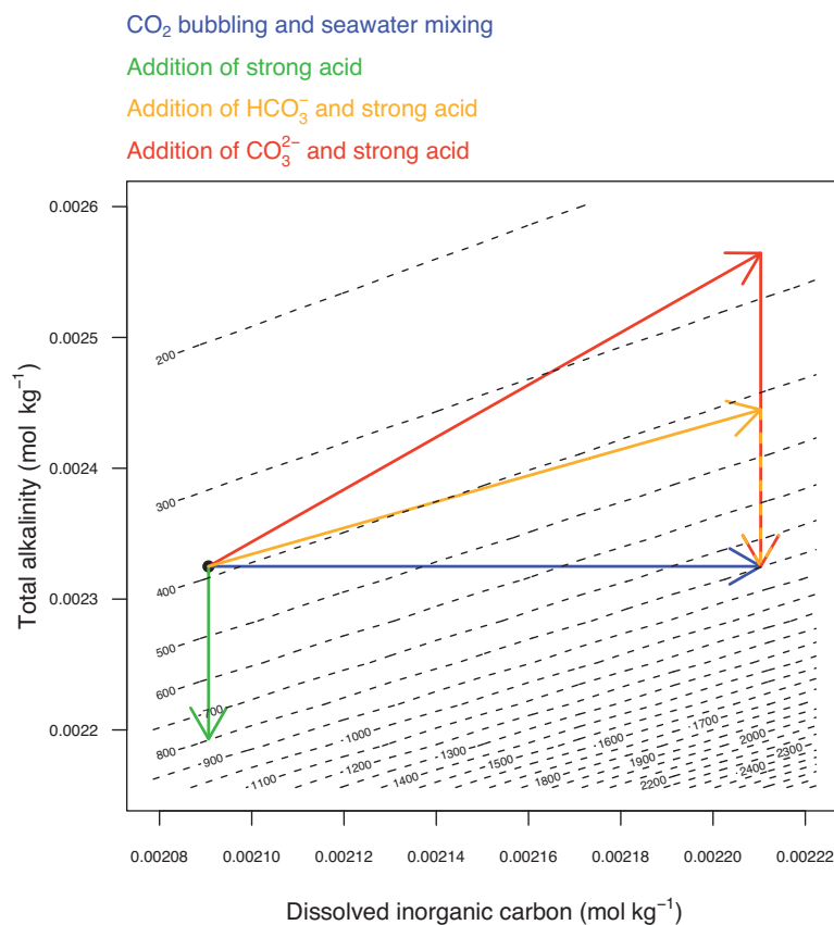
Figure 2.2 Changes in the carbonate chemistry generated by various perturbation techniques, in the A_T vs. DIC space. The plot was generated using the seacarb function \alpha a .
