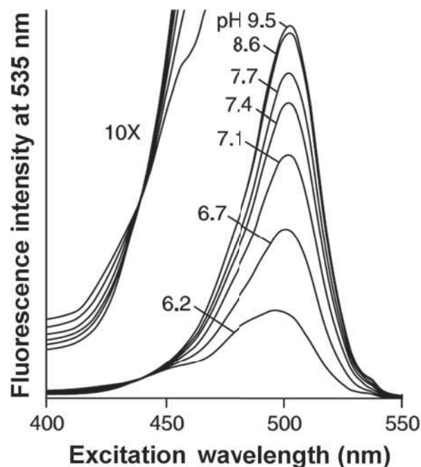
Figure 9.5 Excitation spectrum of BCECF. The curve around the isosbestic point is enlarged 10-fold (upper left). Modified from http://probes.invitrogen.com .
