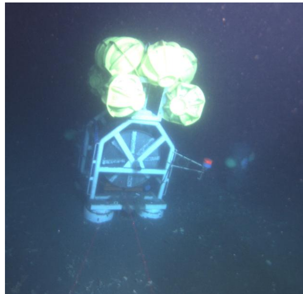
Figure 14. The ROVARD deployment platform, with instruments attached; central spool with cable will facilitate recovery (SSD-placed chimney is back and right).
