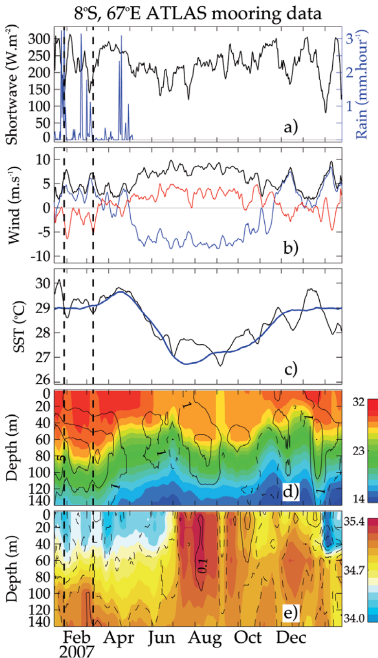
FIG. 6. Time series of daily parameters transmitted by the ATLAS mooring at 8°S, 67°E since its deployment during Cirene. (top to bottom) (a) Downward surface shortwave radiation ( \text{W m}^{-2} ) and rainfall ( \text{mm h}^{-1} ); (b) wind speed (black), zonal wind (blue), and meridional wind (red) ( \text{m s}^{-1} ); (c) SST (black) and SST climatology (blue) ( ^{\circ}\text{C} ); (d) subsurface temperature (color) and anomalies (contours) ( ^{\circ}\text{C} ), and (e) subsurface salinity (color) and anomalies (contours) (psu). The SST climatology in (c) is from TMI (Wentz et al. 2000), and anomalies in (d), (e) are computed with respect to Locarnini et al. (2006).
