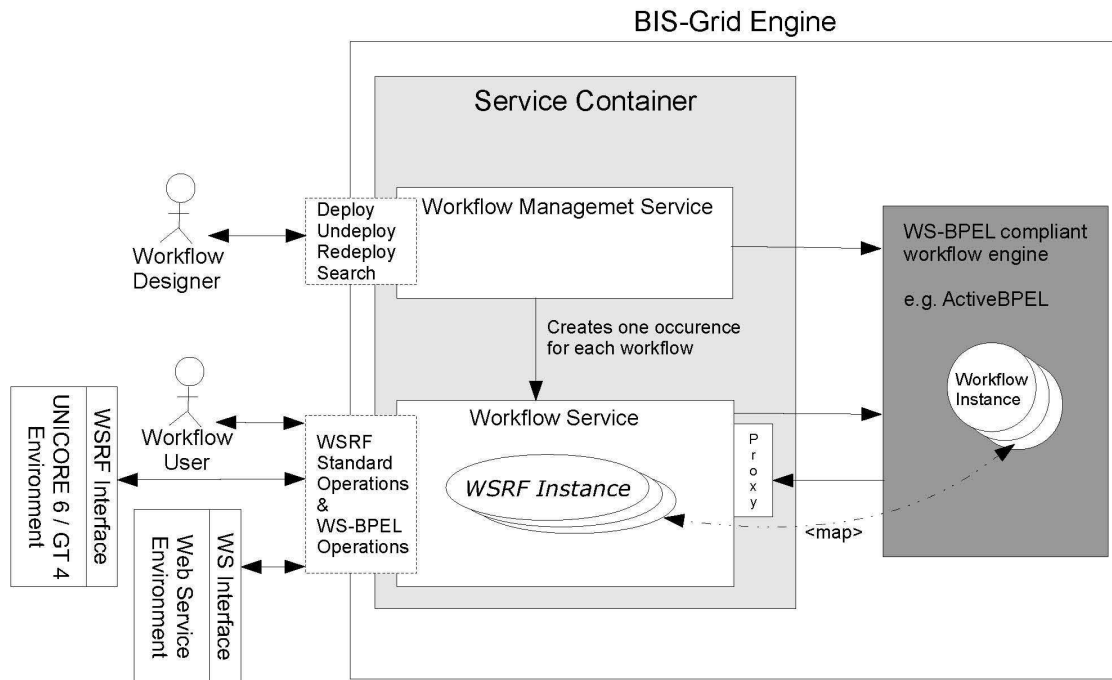
Fig. 2 – BIS-Grid Engine Architecture
