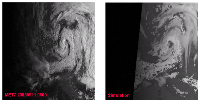
Figure 5. Meteosat 7 image (left) and SIMSAT simulation of the scene based on meteorological data from weather prediction models (right)
