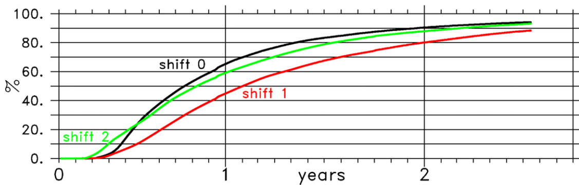
Figure A.2. Total fraction of tracer (in %) outside the western boundary region (30°N to 45°N, 140°E to 160°E, box marked in figure A.1) from three 0.25° model simulations, differing in the initial year of the tracer release.
