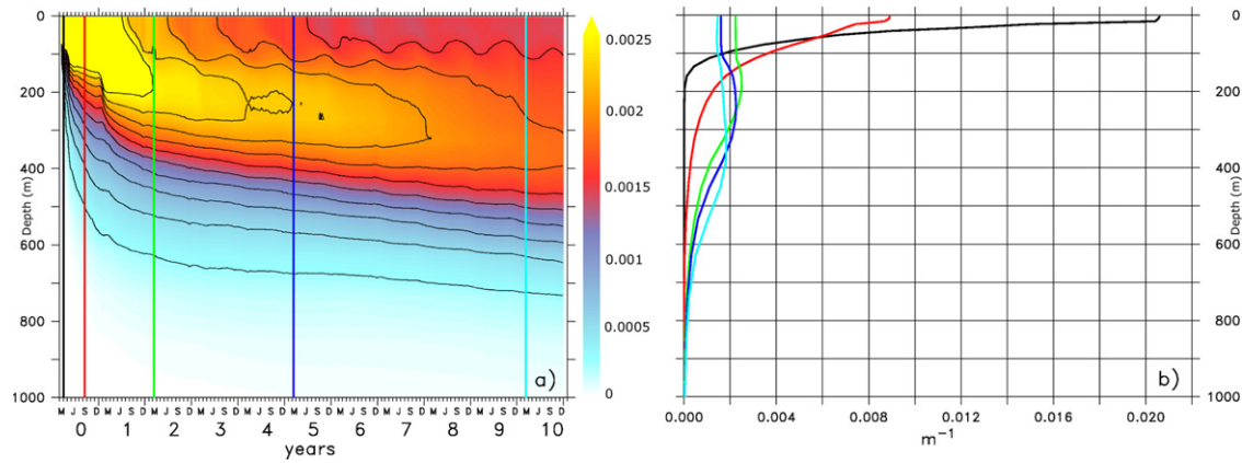
Figure 5. (a) Temporal evolution of relative vertical tracer distribution (in m^{-1} ), horizontally integrated over the North Pacific, from the 0.1^\circ -simulation, contour lines mark a 2.5 \times 10^{-4} interval; (b) vertical profiles from (a) after 15 days (black), 90 days (red), 2 years (green), 5 years (blue) and 10 years (light blue).
