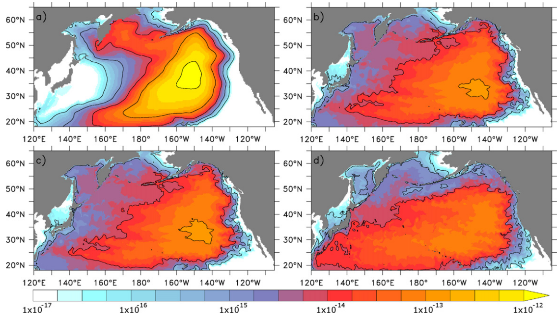
Figure 6. Effect of model resolution and discharge period on relative tracer concentration for the upper 1000 m (in m^{-2} , vertical integral, relative to the tracer inventory in the upper 1000 m, area-standardized) after 5 years for (a) 0.5^\circ -simulation (14 day release period), (b) 0.25^\circ -simulation (14 day release period), (c) 0.25^\circ -simulation (54 day release period), (d) 0.1^\circ -simulation (54 day release period); contour lines mark power of 10 intervals.
