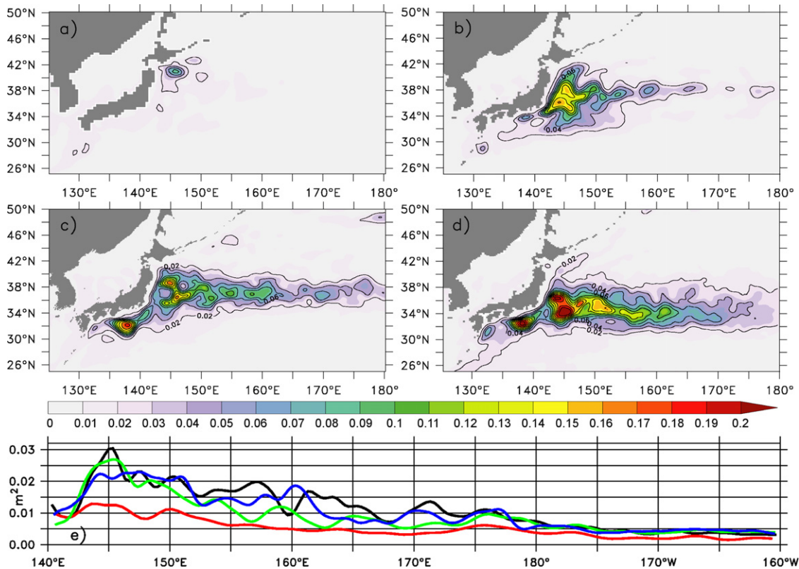
Figure 2. Variance of sea surface height during 1998–2007 (in m^2 ; contour lines indicate a 0.02 m^2 interval) from (a) 0.5^\circ -model, (b) 0.25^\circ -model, (c) 0.1^\circ -model, (d) satellite altimeter data (AVISO) and (e) in a comparison along the axis of the Kuroshio extension (meridionally averaged between 32^\circ N and 40^\circ N ), for AVISO data (black), the 0.5^\circ (red), 0.25^\circ (green) and 0.1^\circ (blue) model simulations.
