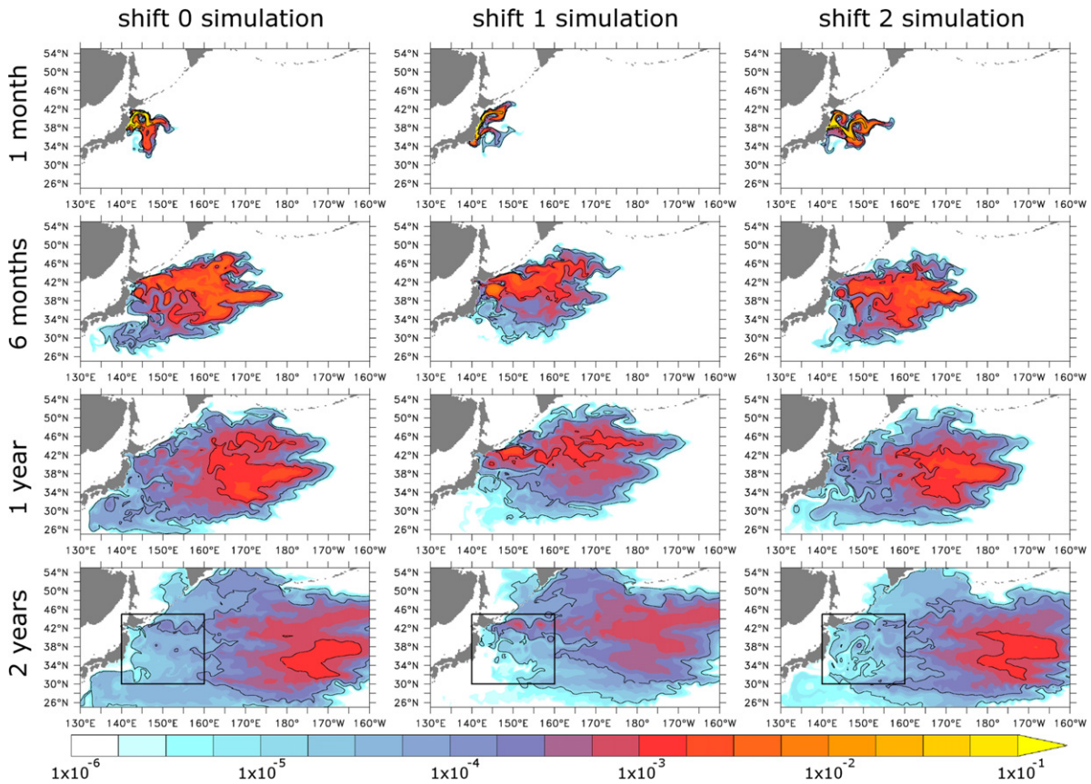
Figure A.1. Sequence of relative surface tracer concentration during the first 2 years, from 0.25° model simulations, differing in the initial year of the tracer release; contour lines mark power of 10 intervals.
