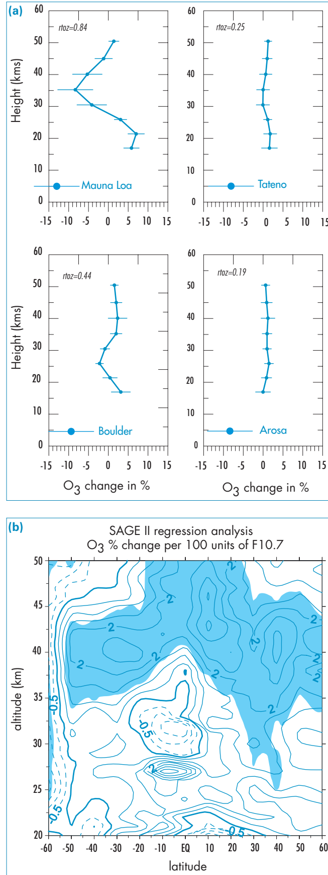
Figure 3. Annual mean ozone response to solar activity in units of percentage change per 100 F10.7 units (recent solar cycle amplitude \sim 130 F10.7 units). (a) Responses at four Umkehr stations for period 1957-2001, horizontal lines show 2-sigma range. (b) Zonal mean response from SAGE II data for the period October 1984-June 2002, contour interval 0.5 %, shading indicates regions of 95 % statistical significance.
