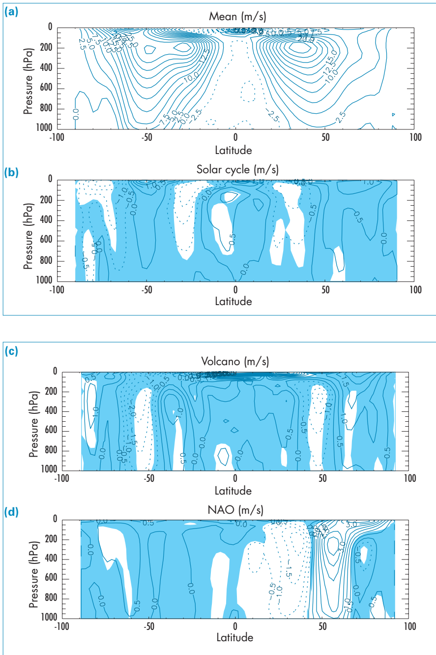
Figure 12. (a) Annual mean, zonal mean, zonal wind (m/s) from NCEP (1979-2002); (b) amplitude of the solar component; (c) volcanic component; (d) NAO. Shaded areas are not statistically significant at the 90% level using a Student's t test. From Haigh et al., 2004.
