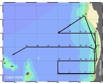
The sampling site of the ATA-03 cruise on the R/V Atalante, 3 rd to 20 th February 2008
