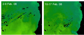
Southward shifting of the upwelling area during the ATA-03 cruise
