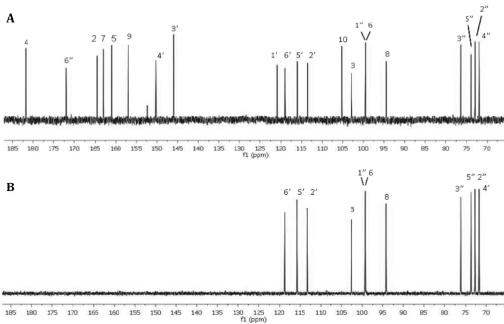
Fig. 7S ^{13}\text{C} -NMR (A) and DEPT-135 (B) spectra of luteolin-7- O -glucuronide ( \text{DMSO-}d_6 , 125 MHz).
