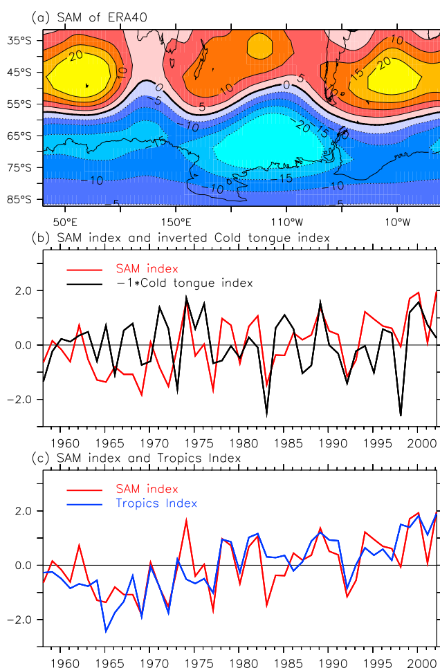
Figure 1. (a) Spatial pattern and (b) time series of the austral summer Southern Annular Mode (SAM) from ERA-40 (1957/1958–2001/2002). The spatial pattern shows the Z500 anomaly corresponding to one standard deviation positive of the index which, in turn, has been normalized by its standard deviation. Also shown in Figure 1b is the inverted cold tongue index (CTI) defined using HadISST data [Rayner et al. , 2003]. (c) Tropics Index (TI), defined as in the text, together with the SAM index from Figure 1b. The units are meters and degrees Celsius in Figure 1a and 1b, respectively, and the Tropics Index in Figure 1c has been normalized by its standard deviation.
