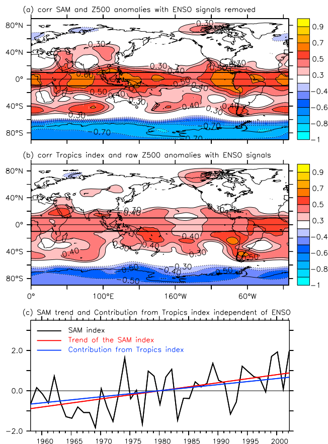
Figure 2. (a) Correlation between the SAM index (see Figure 1) and Z500 anomalies with ENSO removed; (b) correlation between the TI and Z500 anomalies with ENSO included; and (c) the SAM index. Figure 2c also shows the trend of the SAM index (red line) and the SAM trend derived from the TI, as described in the text. In Figures 2a and 2b, detrended data are used for the analysis.
