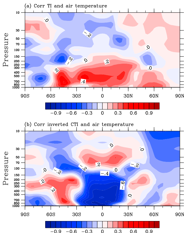
Figure 4. Correlation between seasonal mean (DJF) zonally averaged temperature and (a) the TI and (b) the inverted CTI (all time series detrended). The contour interval is 0.1.
