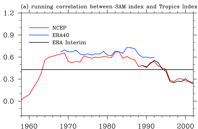
Figure 3. Correlation between the SAM index and the TI (both detrended) in running 21 year windows computed using the NCEP (red line; Kalnay et al. [1996] ), ERA-40 (blue line; Uppala et al. [2005] ), and ERA Interim (black line; [Dee et al., 2011] ) reanalyses. The horizontal black line indicates the 95% significance level.
