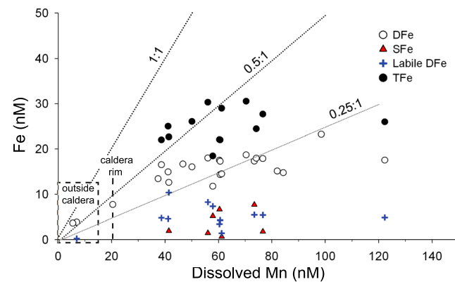
Figure 3. Fe concentrations versus Mn concentration in and outside the Kemp Caldera. Ratios of Fe:Mn are shown as a guide. The focused fluids sampled from the resurgent cone had an Fe:Mn ratio of <0.01, suggesting that a higher Fe:Mn hydrothermal fluid source exists in the caldera. Fluids with Fe:Mn up to 14 have been sampled at other acidic hydrothermal island arcs [de Ronde et al., 2011].
