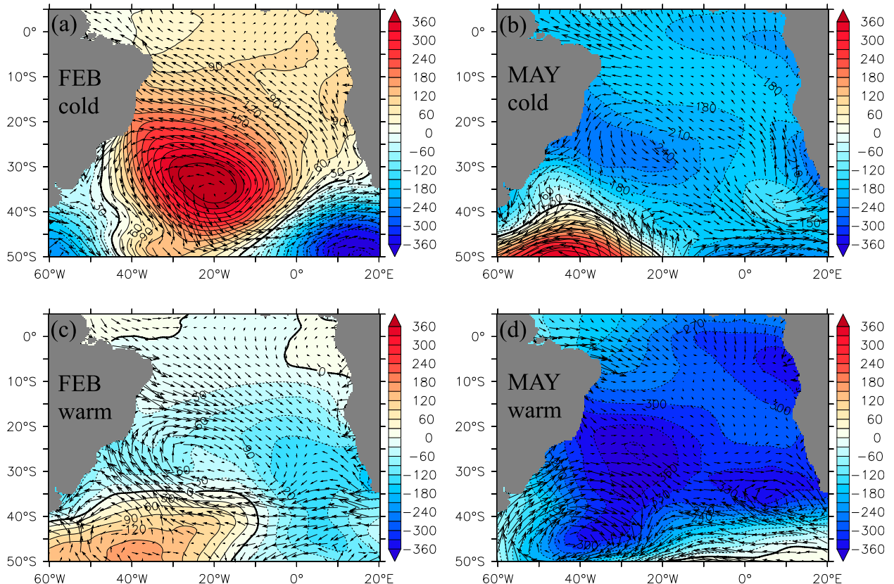
FIG. 7. SLP (hPa) and wind stress anomaly composite from ERA-Interim for (a) February and (b) May of cold strong connection years and (c) February and (d) May of warm strong connection years.
