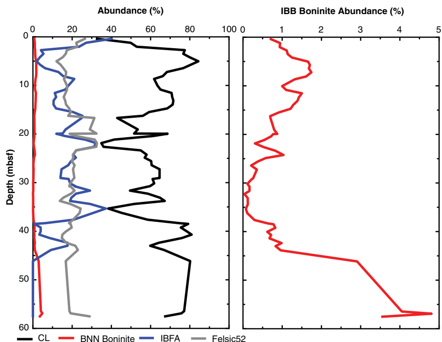
Figure 7. Modeled abundances (wt. %) of end-members contributing to the bulk sediment, Site 52 (supporting information Table S7). Note similarity of the modeled BNN boninite here (expanded view on right) with the Ni/Al ratio of Figure supporting information Figure S7.
