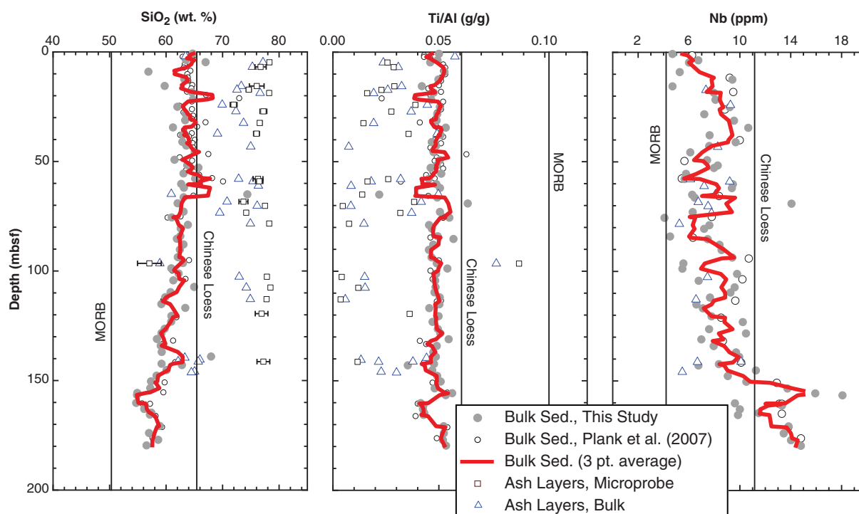
Figure 2. Site 1149, representative compositions (supporting information Table S1) and elemental ratios plotted with depth. Sources for end-member data can be found in supporting information Table S2. Different elemental abundances and ratios suggest contrasting mixtures of representative potential end-member compositions, indicating need for multivariate treatment of large element menu.
