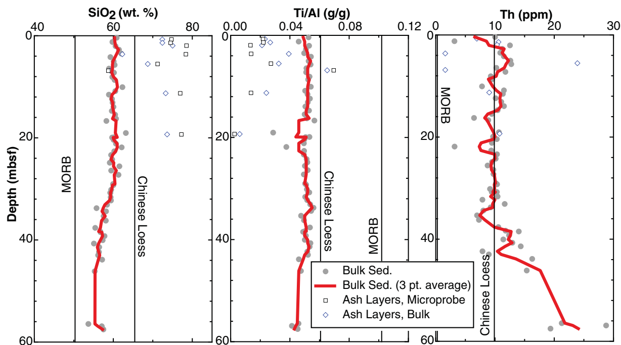
Figure 4. Downcore profiles from Site 52 (data in supporting information Table S1).
