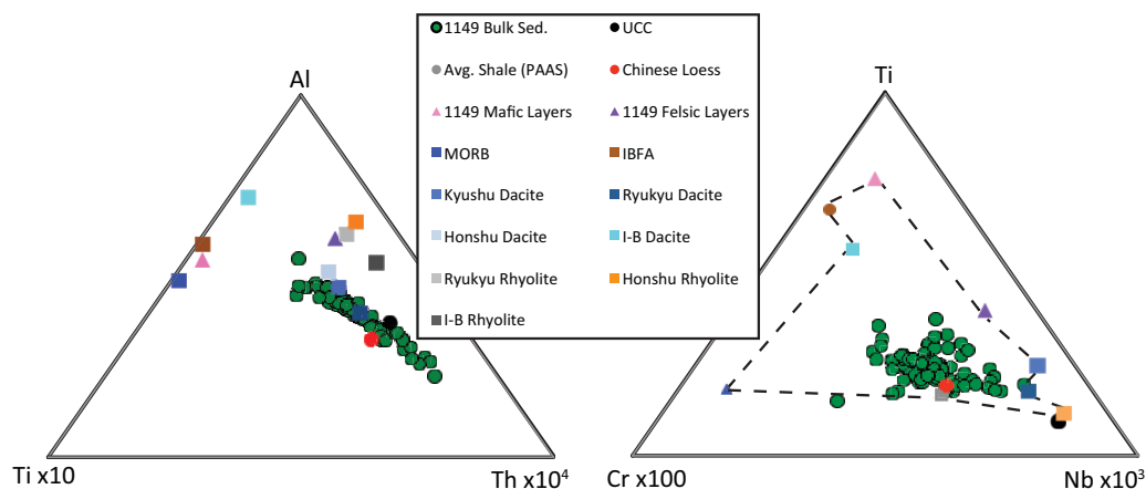
Figure 3. Ternary diagrams showing potential end-members and bulk sediment chemistry at Site 1149. Contrasting patterns indicate a variety of mixing relationships could yield the bulk chemistry. (left) Some of the samples in Unit IIB fall outside the bounds of end-members, particularly toward the Th apex. (right) All samples fall in field circumscribed by all potential end-members.
