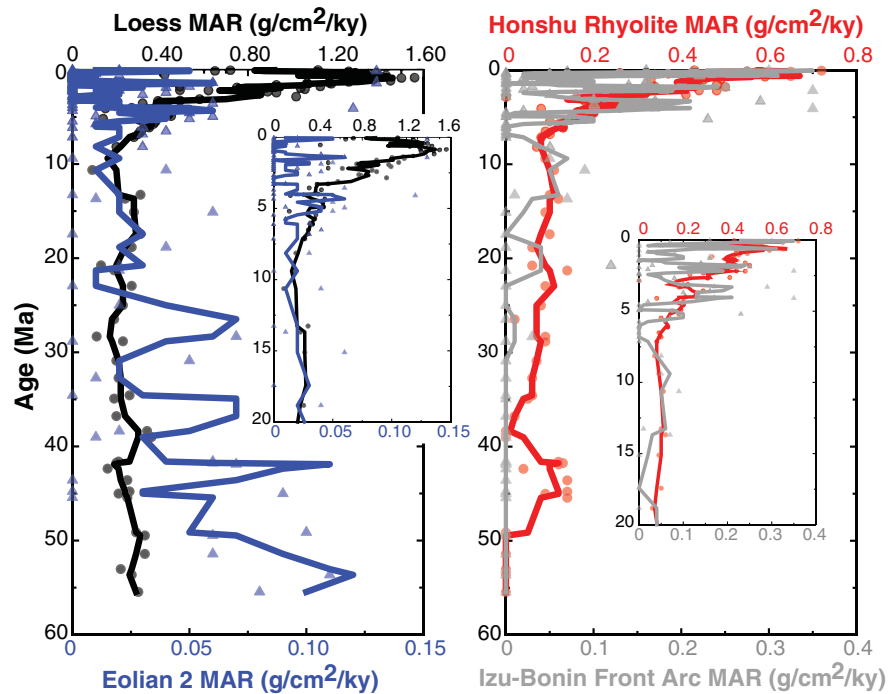
Figure 6. Individual data and three-point averages of MARs of each end-member. Eolian sources on left, dispersed ash on right. Insets focus on the younger portion of each record. Note color-coded different x axis scales and labels. A few dots are covered in left plot by the inset. Data in supporting information Table S7.
