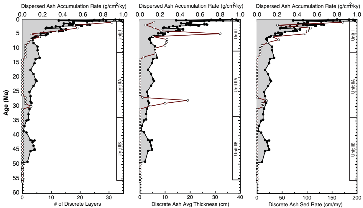
Figure 5. Site 1149. The accumulation rate of total dispersed ash (that is, the accumulation sum of IBFA and HR, gray shaded with filled circles in \text{g}/\text{cm}^2/\text{ky} , and is the same in each plot) plotted against parameters associated with the sedimentation of discrete ash layers per 1 Ma (open circles, and are different in each plot as shown in the bottom x axis labels). Lithologic units plotted on the right in each plot. A moving 1 Ma window was chosen to bin each discrete ash layer parameter to approximate the resolution of the modeled dispersed ash record.
