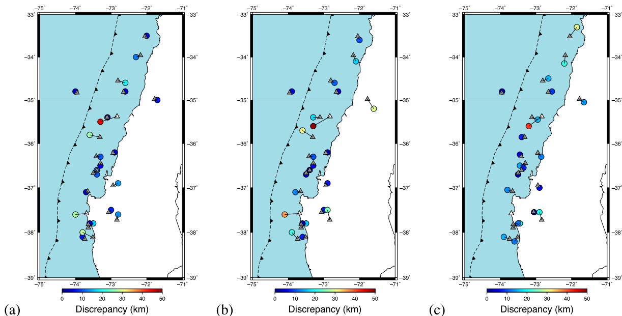
Figure 7. Distance between the epicentres of the calibration aftershocks inferred by backprojection (circles) and by first arrivals recorded by dense seismic local networks (triangles – white triangles mark the NEIC hypocentres). Subplots a, b, c show results for pass bands of 0.4–3, 1–4, 2–8 Hz, respectively.
