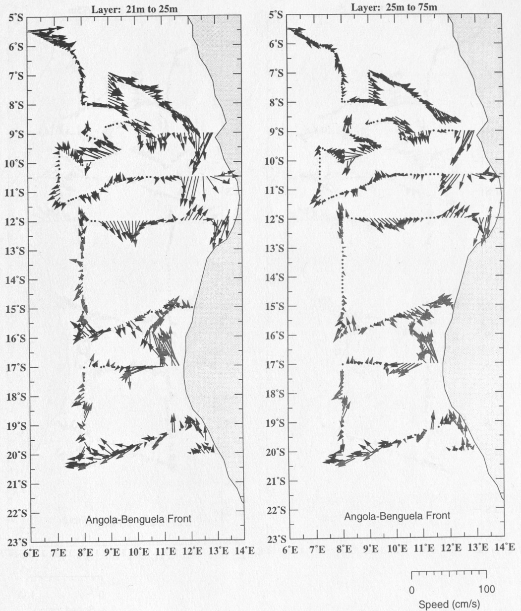
Figure 9.39: Current vectors at 21-25 m level and 25-75 m level, estimated from vessel mounted ADCP measurements. (02. - 28. April 1999)
