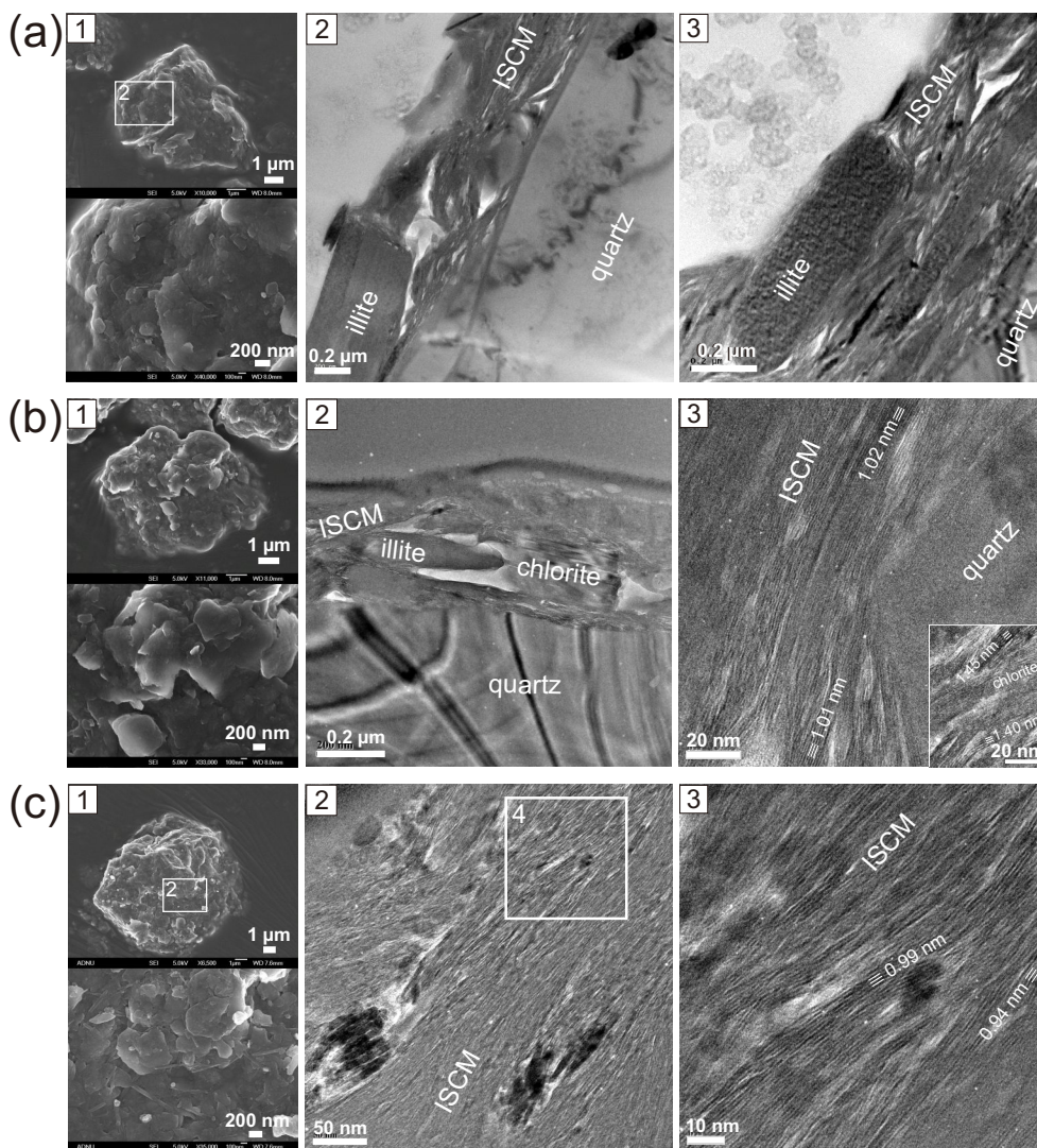
Figure 1. Occurrence of clay minerals in three Asian dust particles ( a , b , c ). Panel 1 in each particle consists of two SEM images of the original particle (low and high magnifications). Panels 2 and 3 are TEM images of the cross-sectional FIB slice prepared from the particle in panel 1.
