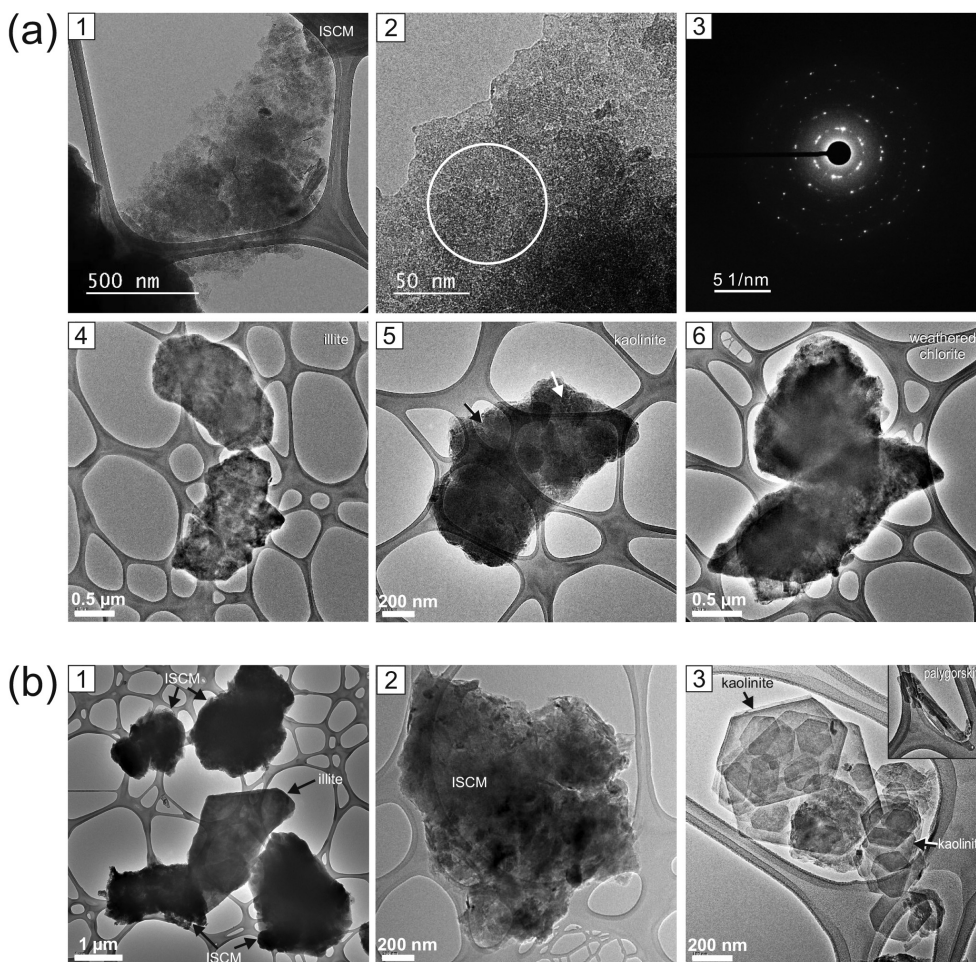
Figure 3. TEM images of clay mineral grains loaded on the micro-grid. Clay mineral grains from Asian dusts, showing ISCM (panel 1), discrete illite (panel 4), kaolinite (panel 5), and chlorite (panel 6) grains. Panel 2 was magnified from Panel 1. Panel 3 is an electron diffraction pattern of the circled area in panel 2 (a). Clay mineral grains from Saharan dusts showing illite (panel 1), ISCM (panels 1 and 2), hexagonal kaolinite (panel 3) and elongated palygorskite (panel 3) grains (b).
