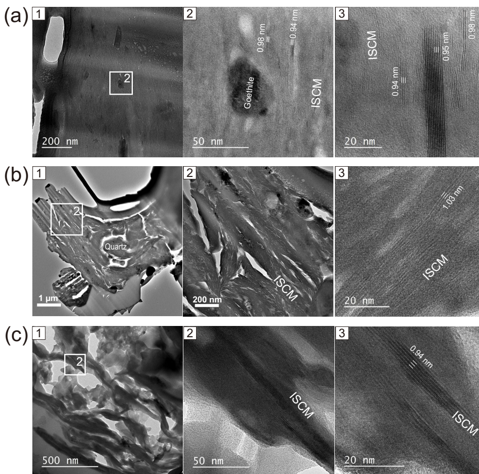
Figure 4. Occurrence of clay minerals in three clay-rich Saharan dust particles (a, b, c). Panel 1 in each particle is a low magnification TEM image of the cross-sectional FIB slice prepared from the original particle. Panel 2 is a TEM image magnified from the TEM image in panel 1. Panel 3 is the lattice fringe image.
