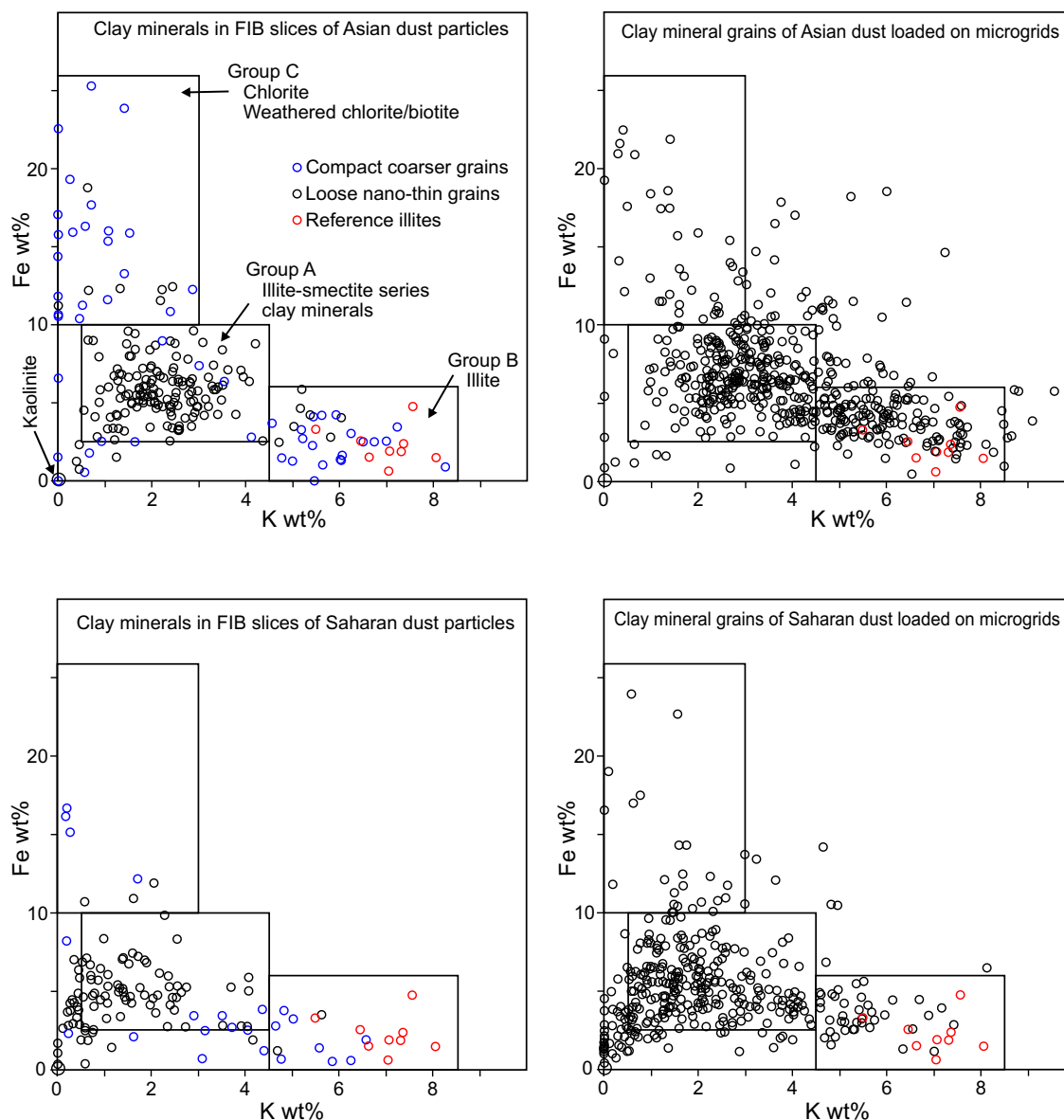
Figure 6. Plots of Fe vs. K from the TEM-EDXS analyses of clay minerals in the cross-sectional FIB slices of dust particles and clay mineral grains loaded on the micro-grids. The boxes indicating groups A, B, and C are drawn on the basis of TEM micro-textures and EDXS data for FIB slices of Asian dust particles.
