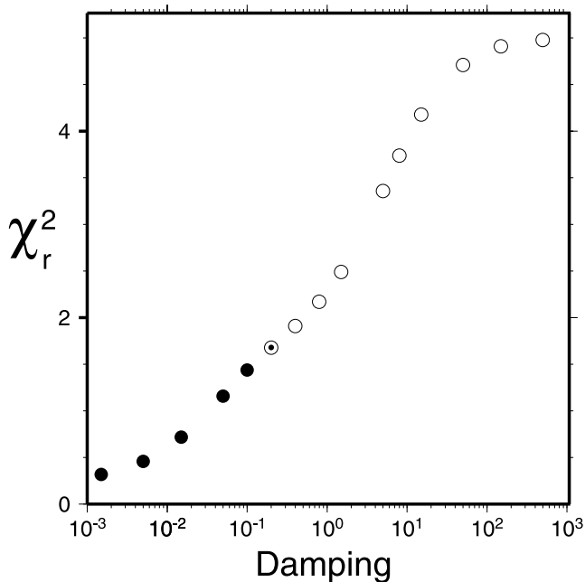
Figure 5. Typical trade-off curve (damping versus misfit, \chi_r^2 ) for the inversion process. Largest damping value ( 10^3 ) gives uniform slip solution. Damping values smaller than 10^{-1} (solid circles) result in low misfit solutions but have negative slip on the fault plane, which may be physically unreasonable. Circled dot represents damping value used for most results in this study.
