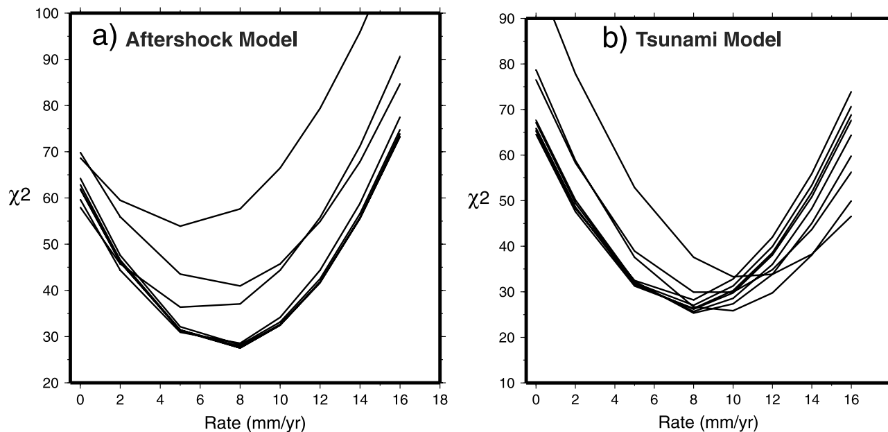
Figure 10. Misfit ( \chi^2 ) versus trench-parallel translation rate for the Nicoya block, for 10 low misfit models of postseismic response from the 1992 Nicaragua tsunami earthquake (see Figure 9). (a) Fault plane defined by aftershocks. Best fit model has viscosity of 10^{19} Pa s (lower crust) and 10^{20} Pa s (upper mantle), fault slip 3–5 m; models with upper mantle viscosity of 10^{19} Pa s fit the data nearly as well. (b) Fault plane defined by tsunami model. Best fit model has viscosities of 10^{18} Pa s (lower crust) and 10^{20} Pa s (upper mantle) and fault slip of 3 m; models with lower crust and upper mantle viscosities of 10^{18} and 10^{19} Pa s, respectively, and fault slip of 1m fit the data nearly as well. There is a well-defined minimum at 8 mm/yr regardless of earthquake or rheological model. Uncertainty can be estimated by arbitrarily taking \chi^2 value 10% larger than the minimum \chi^2 , giving \pm 3 mm/yr.
