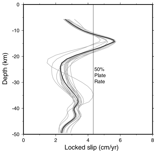
Figure 14. Similar to Figure 13, showing sensitivity of inversion to data at individual GPS sites. Best fit postseismic model and block translation rate are assumed. Successive data points in the Nicoya region are eliminated, and the data are reinverted. For 17 starting data we perform 16 separate inversions using 16 data (thin grey lines) compared to best fit results using all 17 data (heavy solid line).
