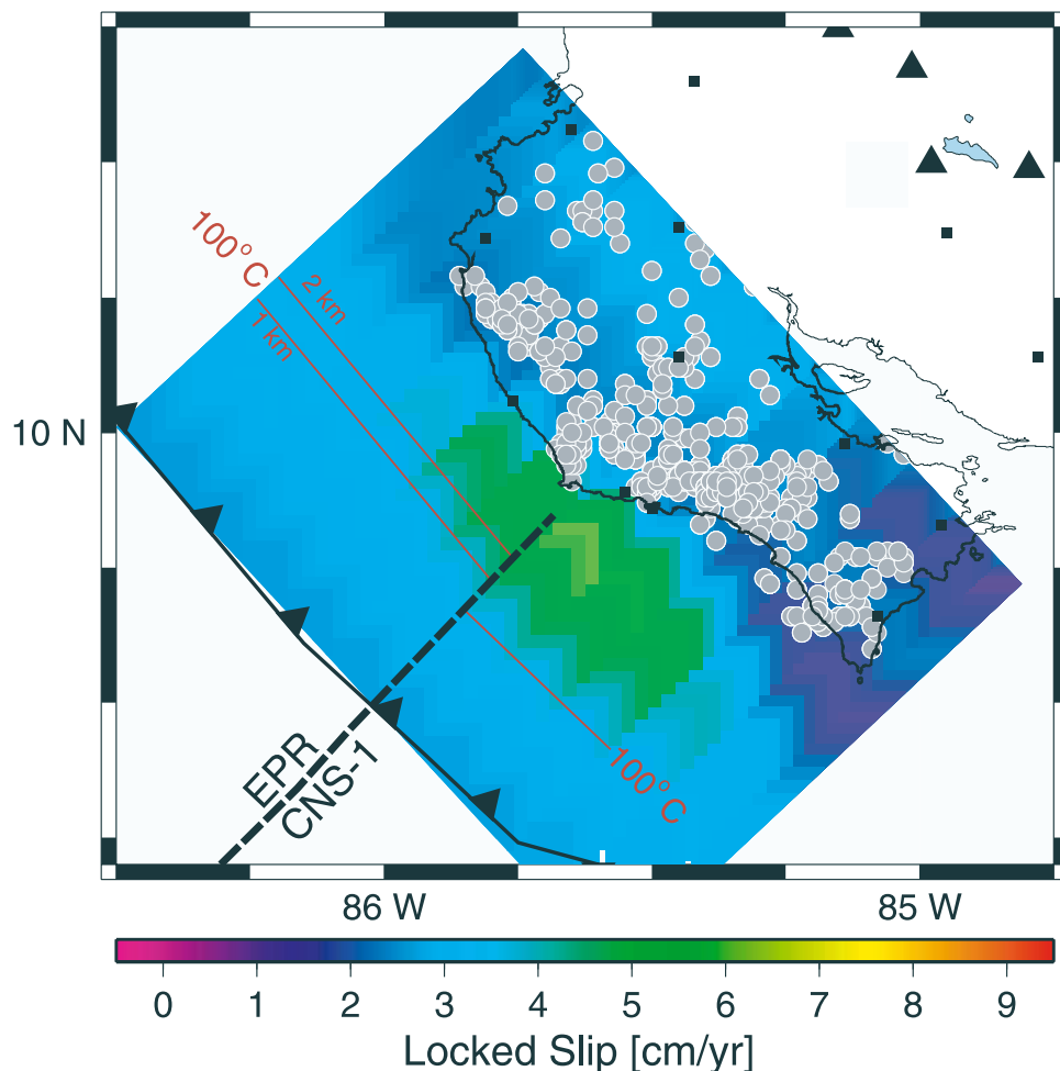
Figure 17. Comparison of well-located earthquakes from our seismic network, distribution of locking from inversion of GPS data, and 100°C isotherms from Spinelli and Saffer [2004]. For East Pacific Rise (EPR) crust, this is calculated assuming hydrothermal cooling of upper 1 and 2 km. Black triangles are active volcanoes. Earthquakes reach an updip limit about 50 km from the trench; maximum locking is centered about 35 km from the trench, approximately coincident with the 100°C isotherm that abruptly shallows across the boundary between crust generated at the EPR and Cocos-Nazca Spreading Center (CNS-1).
