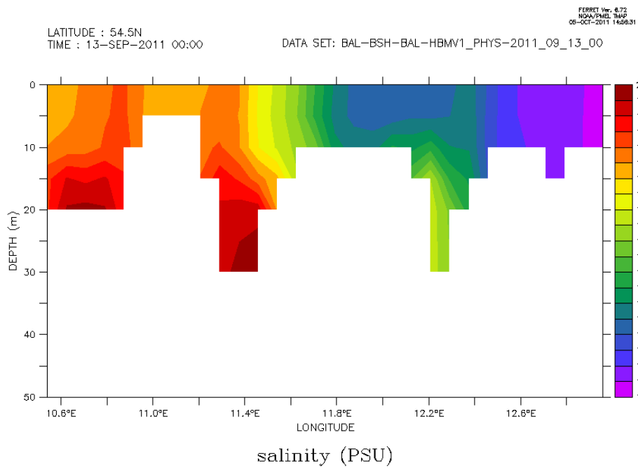
Figure 4.9: Temperature (above) and salinity (below) along the L section as represented in the BSH model (data kindly provided by F. Jansen/T Brüning, BSH, Hamburg).
