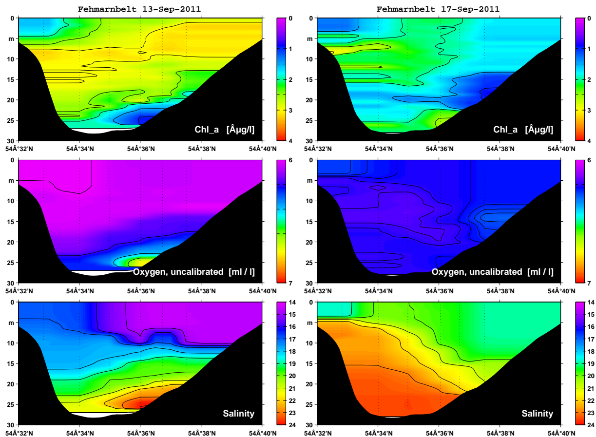
Figure 4.6: Chlorophyll, oxygen and salinity distribution along Fehmarn Belt. Left: 13. Sept. 2011; right: 17. Sept. 2011
