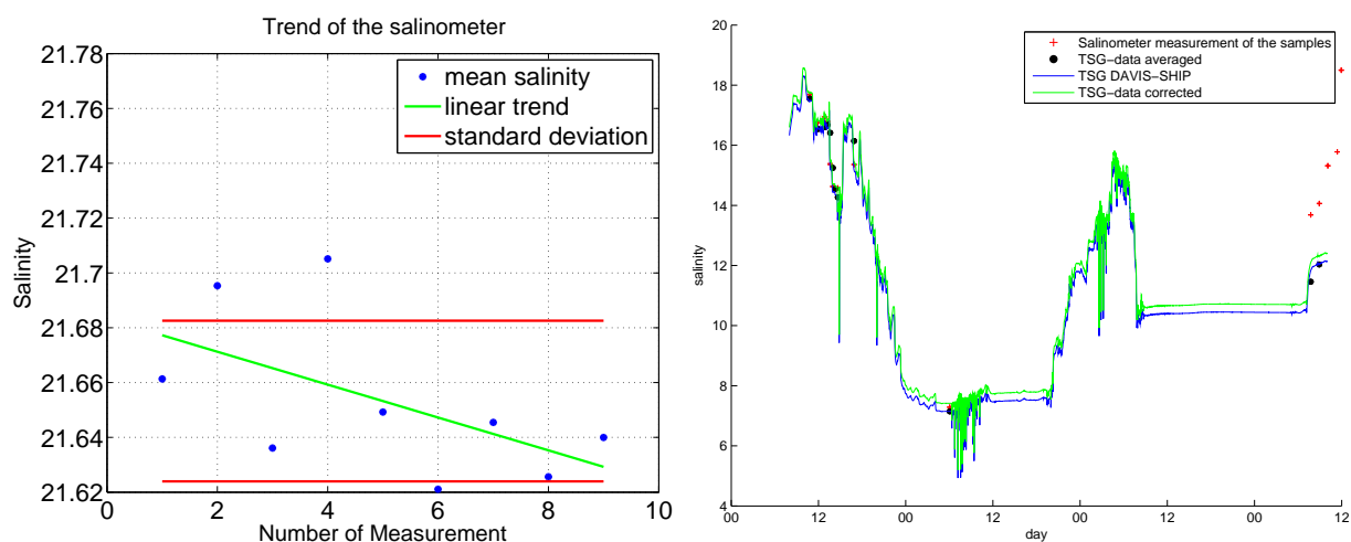
Figure 5.4: (left) Trend of the salinometer based on Substandard measurements. (right) Observations from the Thermosalinograph.
