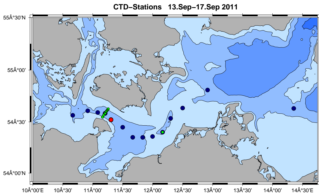
Figure 3.1: ALKOR 33/11 cruise stations. Black (LG section)/ Green (FB section) and Red dot are the CTD stations, red dot is also location of the V431 mooring.
