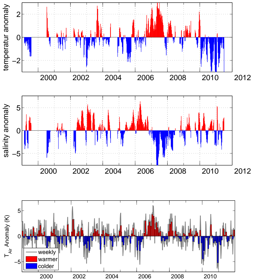
Figure 5.3: (upper) temperature and (middle) salinity anomaly based on all available data between 1999 and 2011. (lower) Air-temperature anomalies derived from daily data from Station Westermarkelsdorf (Fehmarn) provided by DWD via website. Anomalies based on weekly averages (gray line) and monthly averages (bars) are shown.
