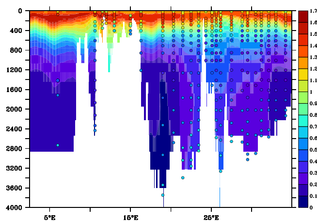
Figure 4. CFC-12 ( pmol\ kg^{-1} ) data–model comparison along the Meteor M51/2 section. Color-filled contours indicate simulated CFC-12, whereas color-filled dots show in situ observations. Both use the same color scale and are taken at the same time (November 2001).
