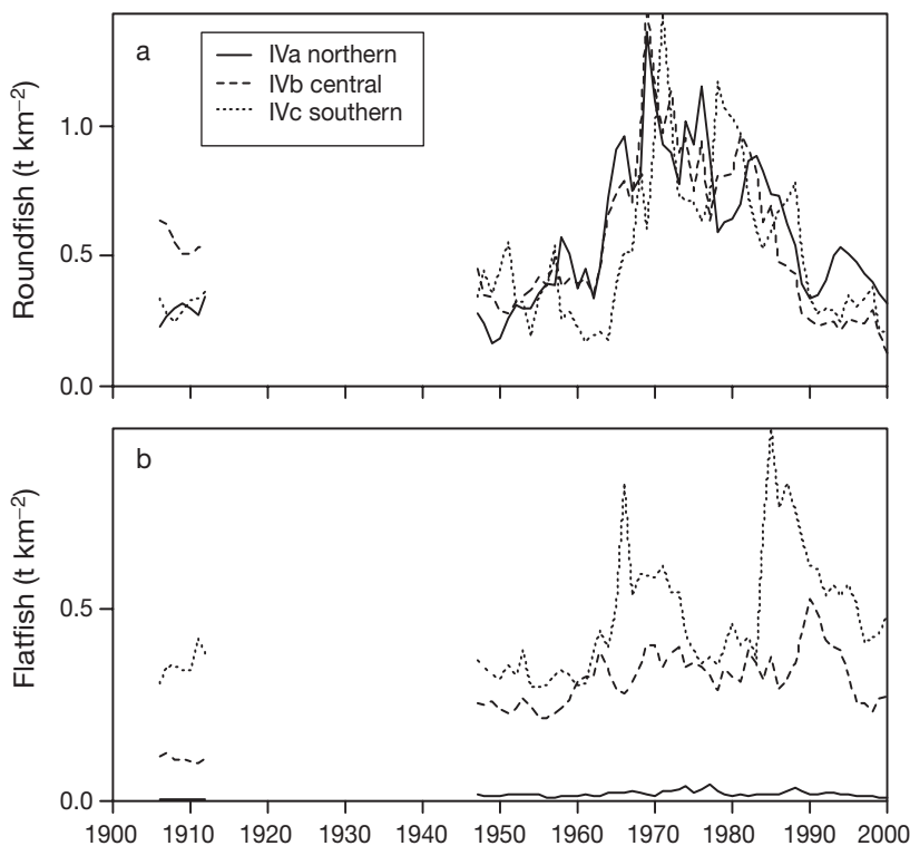
Fig. 3. Long-term changes in landings per area of (a) roundfish and (b) flatfish for the northern, central and southern North Sea throughout the 20th century (no data by ICES division for 1913 to 1946)
