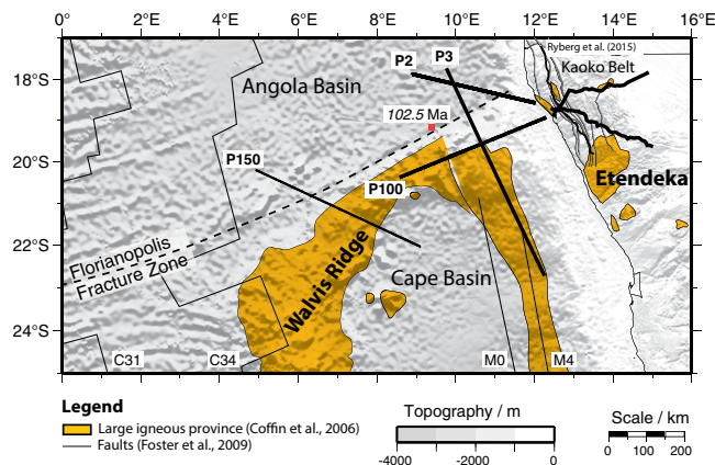
Figure 1. Location of the deep crustal seismic profiles at the Walvis Ridge, southeast Atlantic Ocean. Magnetic anomalies with the ages (Gee and Kent, 2007): C34, 83.5 Ma; M0, 120.6 Ma; M4, 125.7 Ma. Red square marks the dated Deep Sea Drilling Project Site 530 Leg 75 in the Angola Basin (Shipboard Scientific Party, 1984).
