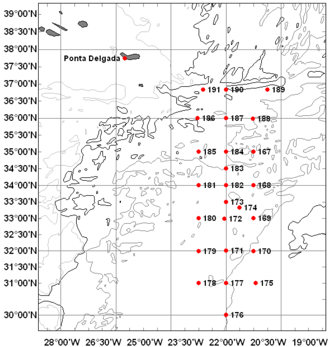
Fig. 1: Cruise track of POS485 in Mai 2015 from Malaga (Spain) to Ponta Delgada (Portugal). Numbers indicate the positions of hydrographic stations (CTDs). The cruise started in Malaga (Spain) and ended in Ponta Delgada (Portugal).
