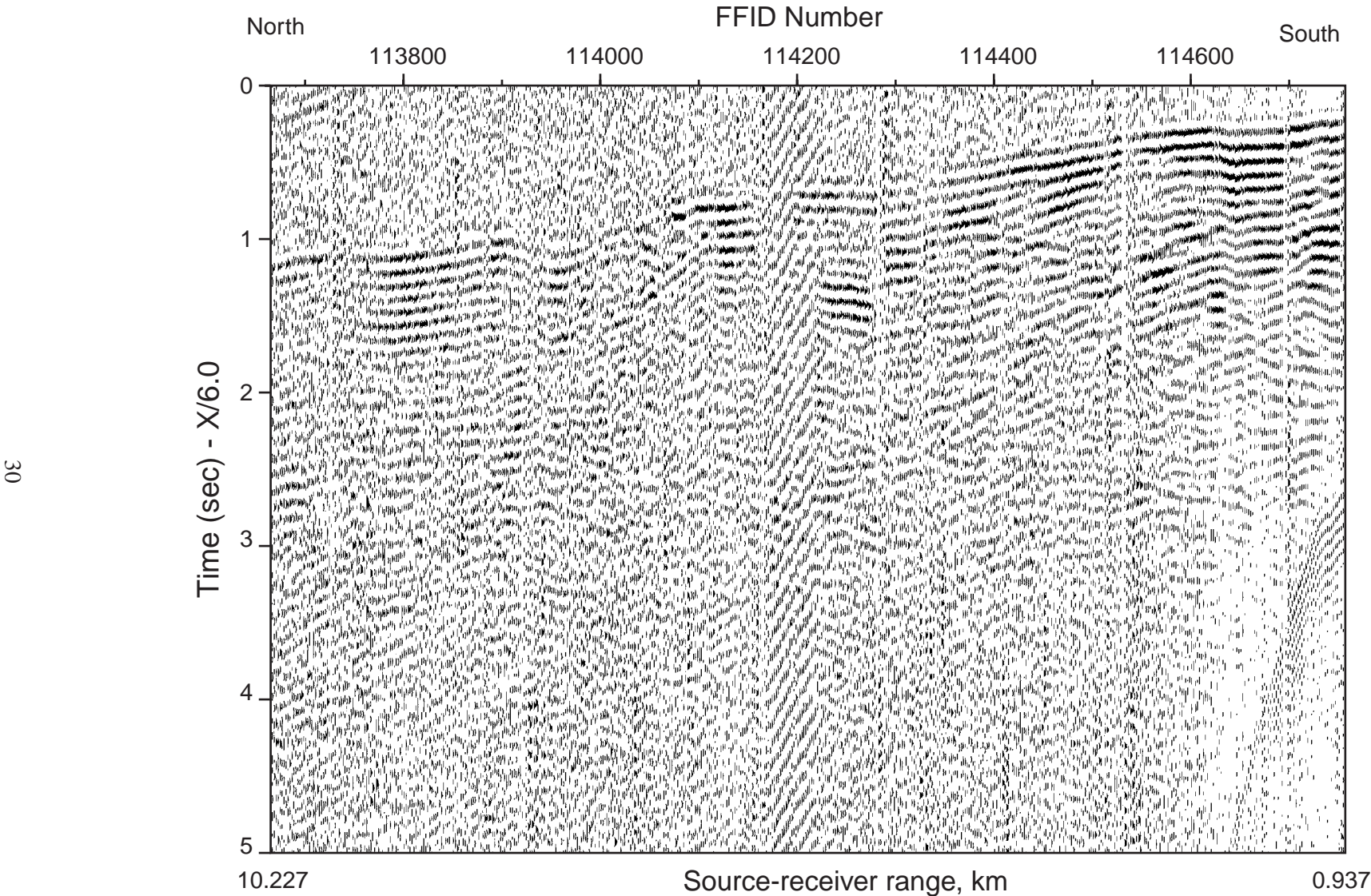
Figure 5. Common-receiver gather for site 151 (DAS 7284), for line 4, Julian Day 135. Traces have been bandpass filtered and only every other trace is plotted. Line 4 is a line running along the north end of Orcas Island.
