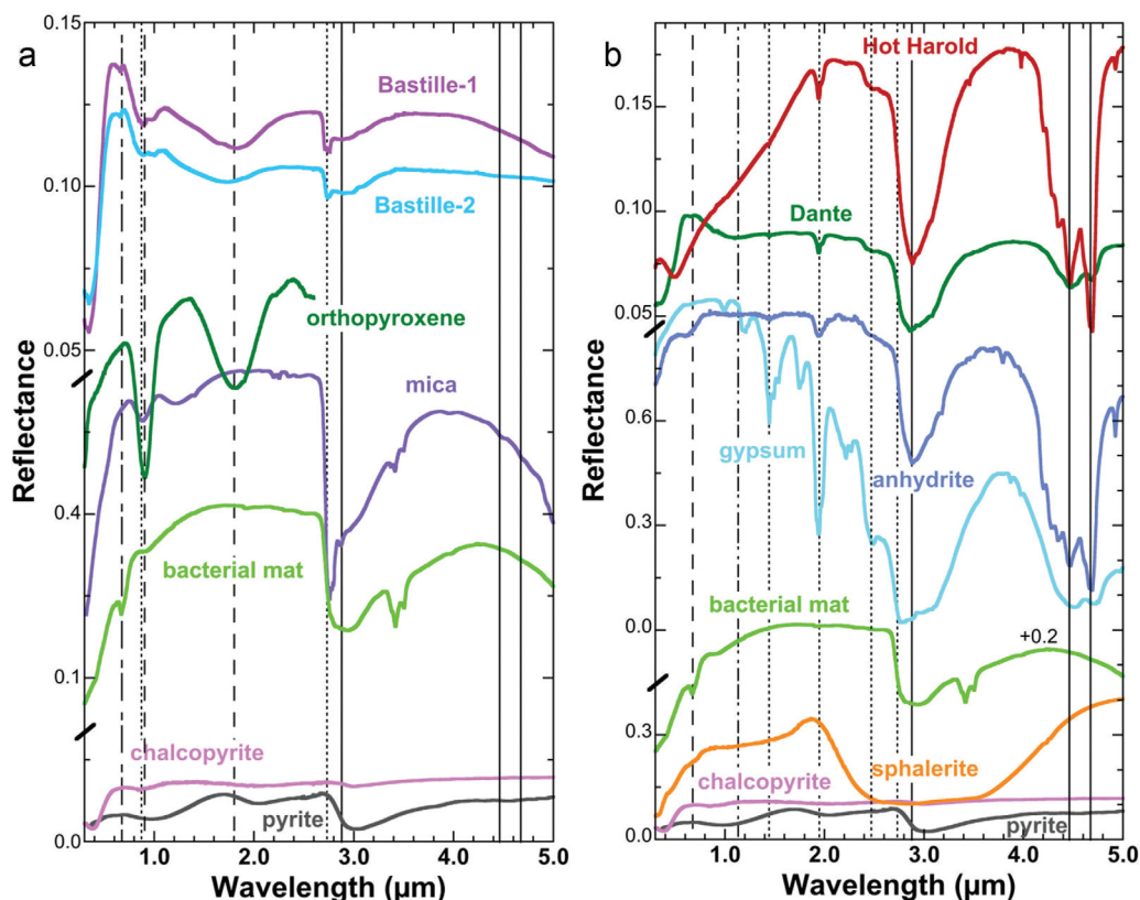
Figure 5. Reflectance spectra are shown from 0.35 to 5 \mu\text{m} for the Bastille, Dante, and Hot Harold samples together with spectra of likely minerals present in the samples. (a) VNIR spectra of Bastille-1, Bastille-2, orthopyroxene DL064 [Klima et al. , 2007], zinnwaldite mica JB729 [Bishop et al. , 2008], JB205, a chlorophyll-bearing bacterial mat from beneath Lake Hoare in the Antarctic Dry Valleys [Bishop et al. , 2001], chalcopyrite HS431 [Clark et al. , 2007], and pyrite GDS483 [Clark et al. , 2007]. (b) VNIR spectra of Hot Harold, Dante, anhydrite GDS42 [Clark et al. , 2007], gypsum JB567 [Bishop et al. , 2014], chlorophyll-bearing mat JB205, sphalerite HS136 [Clark et al. , 2007], chalcopyrite HS431, and pyrite GDS483.
