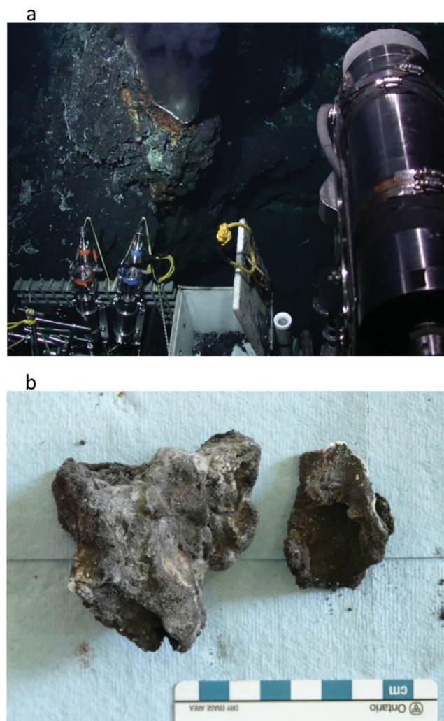
Figure 4. Hot Harold chimney sample. (a) Hydrothermal chimney actively venting 321°C fluid as seen on the seafloor prior to collection. (b) The hydrothermal chimney fragments as seen on board ship prior to subsampling.
