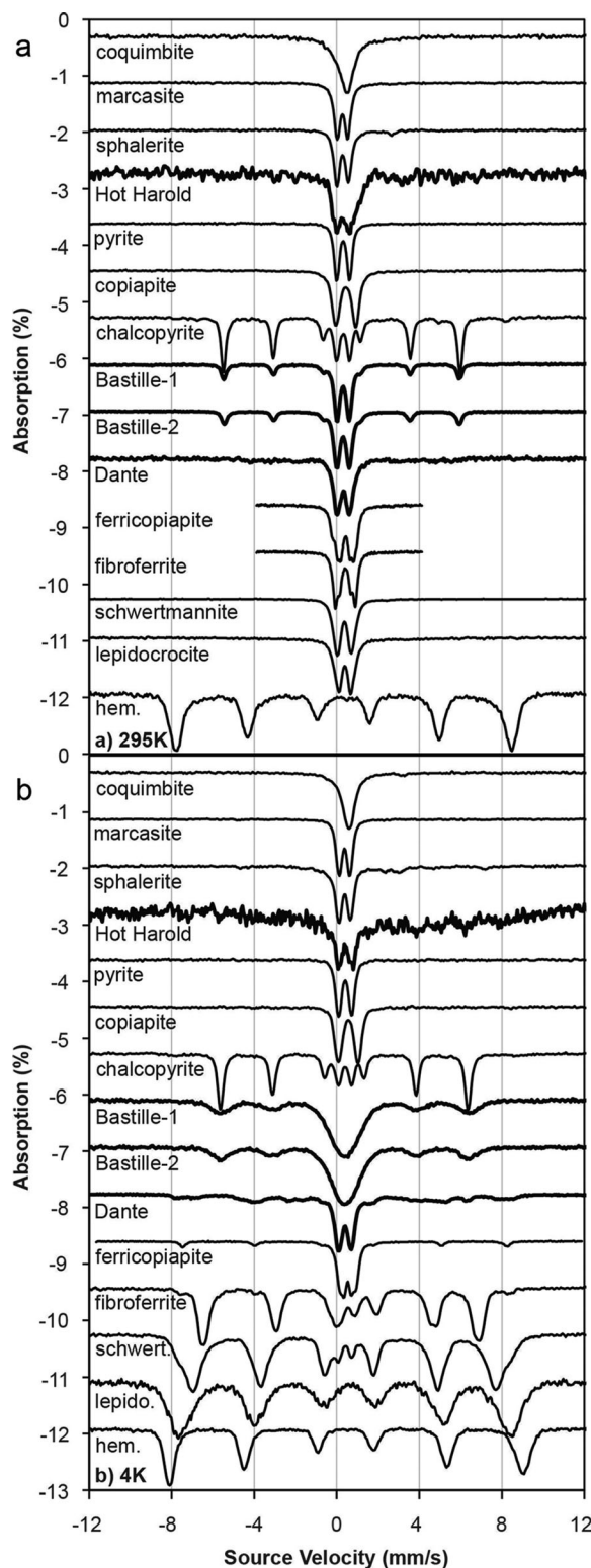
Figure 7. (top) Mössbauer data acquired at 295 K and (bottom) 4 K. Hydrothermal samples are shown with similar minerals. The spectra of Bastille consist of a chalcopyrite sextet and a doublet that could be pyrite, sphalerite, or marcasite. The Dante spectra contain a doublet that could represent pyrite, sphalerite, or marcasite and a sextet that could be ferricopiapite, lepidocrocite, or schwertmannite. The Hot Harold sample had too little Fe to produce an interpretable Mössbauer spectrum.
