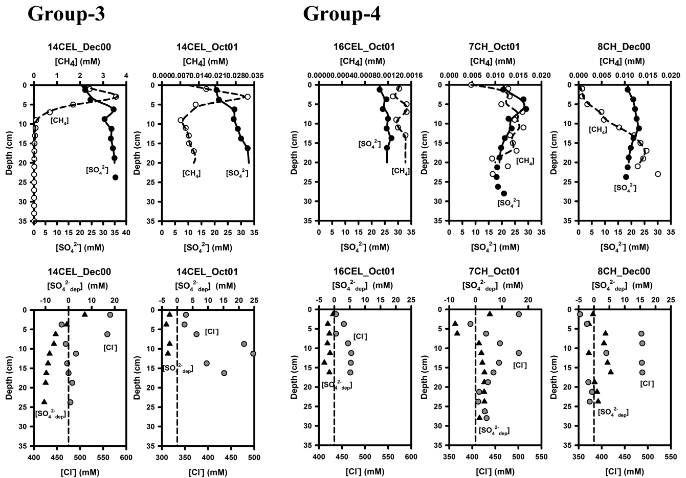
Figure A1. Depth profiles of modeled (lines), measured (circles) and calculated (triangles) concentration of dissolved methane (dashed lines; open circles), sulfate (solid lines; solid circles) in the upper panel and sulfate depletion (solid lines; solid triangles), zero sulfate depletion (dashed lines) and chloride (gray circles) in the lower panel for each profile type (Groups 1–4, see text). One selected profile per group is shown in Fig. 2 for illustration and here the other profiles are shown (9 cores for Group-1, 6 cores for Group-2, 2 cores for Group-3 and 3 cores for Group-4). CEL and CH represent cores collected from Celestún Lagoon and Chelem Lagoon.
