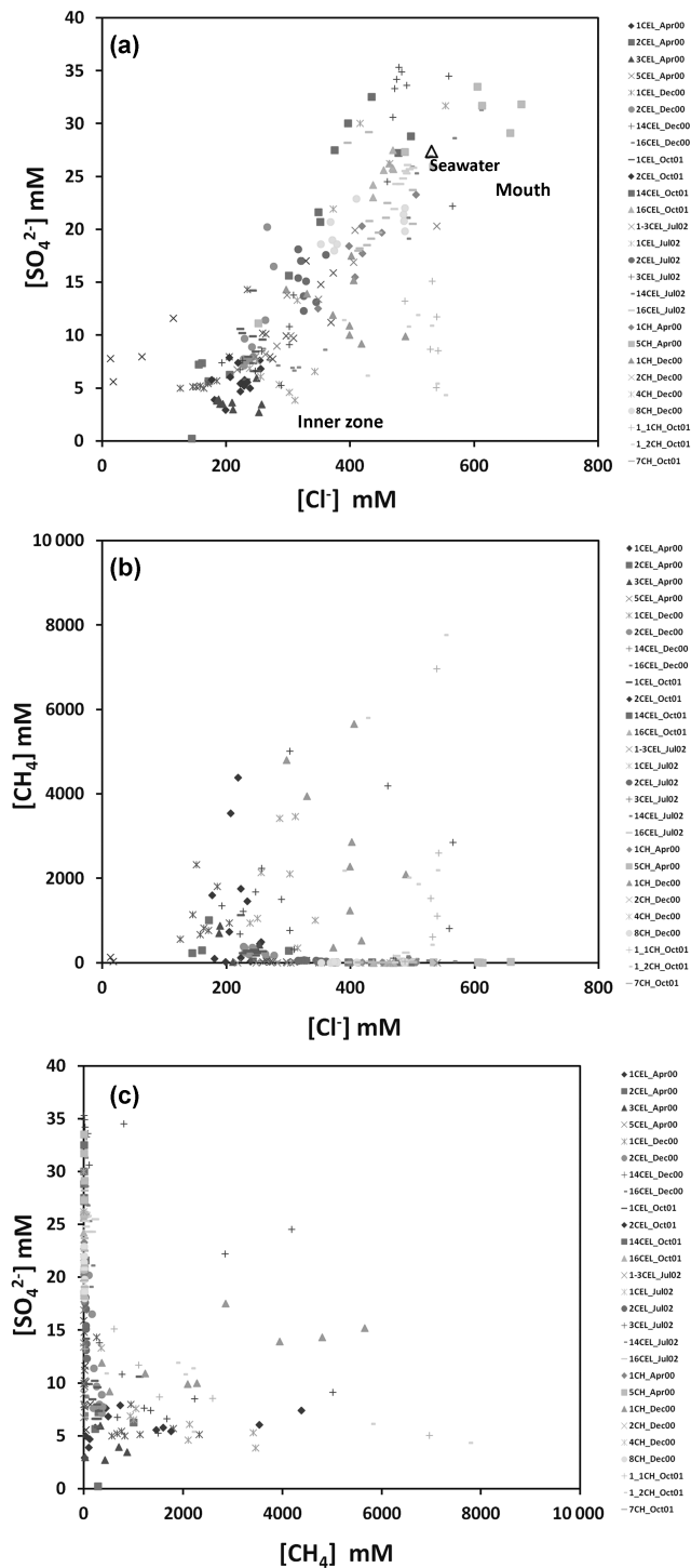
Figure 3. Relationship between (a) [\text{Cl}^-] and [\text{SO}_4^{2-}] , (b) [\text{Cl}^-] and [\text{CH}_4] and (c) [\text{CH}_4] and [\text{SO}_4^{2-}] in porewater samples.
