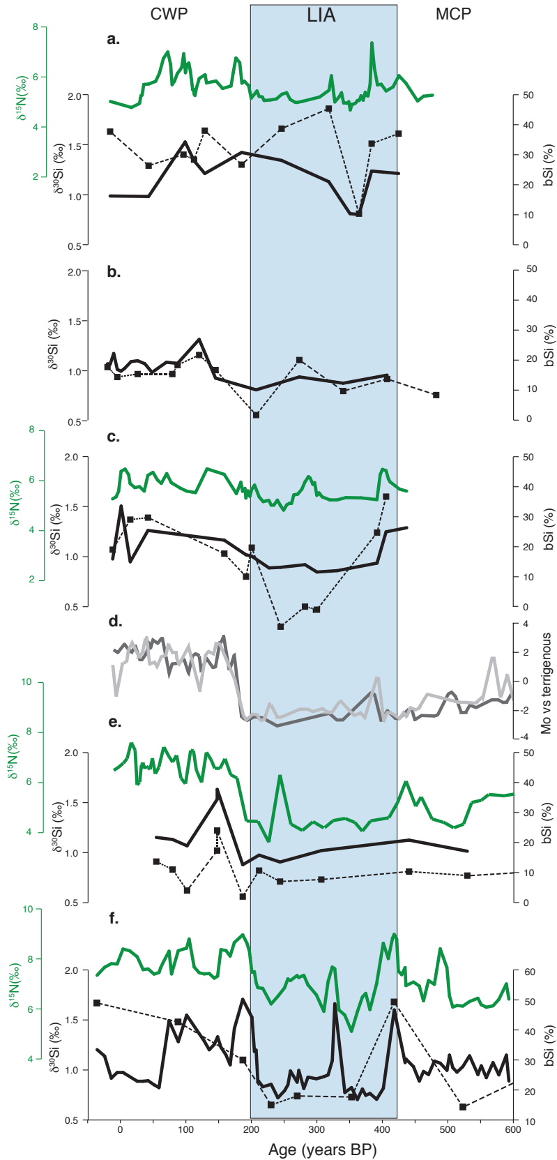
Figure 2: Downcore comparison for \delta^{15}\text{N} (‰), bSi (%), \delta^{30}\text{Si} (‰) and Mo vs terrigenous of cores: a.) M77/2-024-5TC, b.) M77/1-470 [Ehler et al. , 2015], c.) M77/2-005-3TC, d.) BO405-13 and -6 [Sifeddine et al. , 2008], e.) B0405-6 [Ehler et al. , 2015; Gutierrez et al. , 2009] and f.) M77/2-003-2TC.
