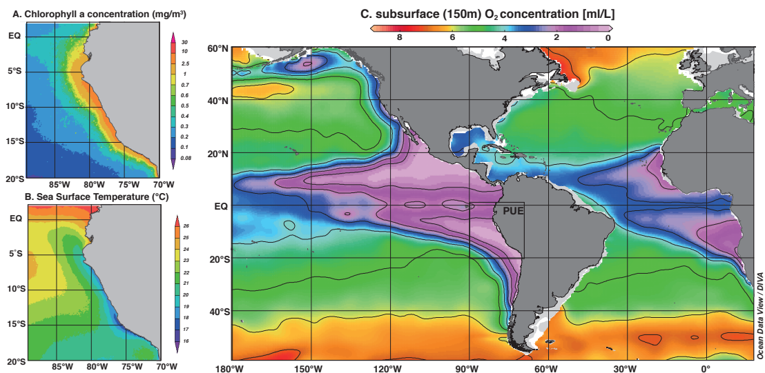
Figure 1.5: Maps of A. Chlorophyll a concentration ( \text{mg}/\text{m}^3 ); B. Sea Surface Temperature ( ^{\circ}\text{C} ), averaged for the period between 1997 and 2015 ( http://oceancolor.gsfc.nasa.gov/cgi/l3 ); C. Dissolved oxygen concentration ( \text{ml}/\text{L} ) at 150m water depth in the Eastern Pacific and the Atlantic; the area of the Peruvian Upwelling Ecosystem (PUE) is highlighted.
