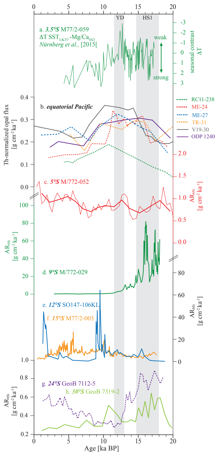
Figure 6: Downcore comparison of a. Difference between UK' 37 and Mg/Ca SSTs given as \Delta T SST UK' 37 -Mg/Ca of core M77/2-059 [Nürnberg et al., 2015];, biogenic opal fluxes from the EEP (b.; [Bradtmitter et al., 2006, Kienast et al., 2006b; Pichevin et al., 2009; Dubois et al., 2010]) the Peruvian Upwelling System (c-f; this study [Ehlert et al., 2013; Schönfeld et al., 2015; Doering et al., 2016]) and the Chilean Coast (g and h ; [Mohtadi, 2004]) over the past 20,000 years. Accumulation rates for the EEP and the Southern Chilean Coast (PC1 and PC3) are given as 230 Th-normalized opal fluxes, while the records from the Peruvian Upwelling System and Northern Chilean Coast (GeoB 7112 and 7319) were calculated without 230 Th-normalization and were calculated from opal content, sedimentation rates and dry bulk densities. All values are given in g cm -2 ka -1 .
