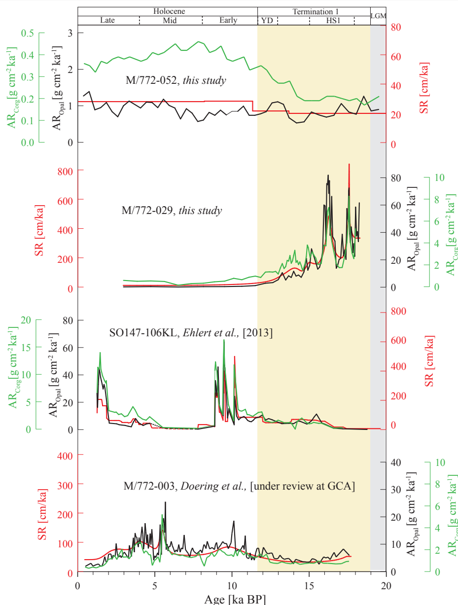
Figure 2: Time series of sedimentation rates [red lines; \text{cm ka}^{-1} ], accumulation rates of biogenic opal (black lines) and organic carbon (green lines) [ \text{g cm}^{-2} \text{ka}^{-1} ] of cores M77/2-52, M77/2-29, SO147-106KL and M77/2-003. Note the different scales of the records of each core.
