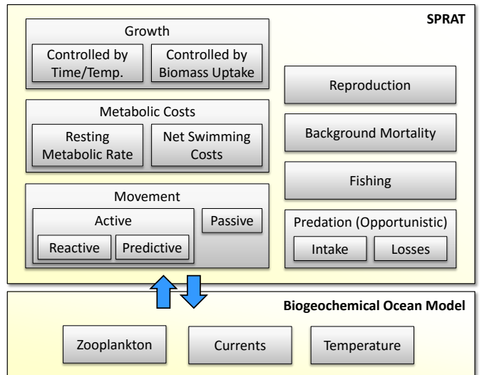
Figure 1: Conceptual diagram of the SPRAT model.
