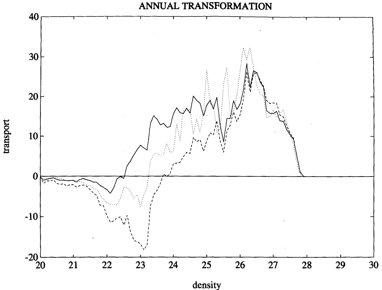
FIG. 2. Annual transformation ( 10^6 \text{ m}^3 \text{ s}^{-1} ) versus sea surface density ( \text{kg m}^{-3} ) over the North Atlantic: comparison of Isemer and Hasse (1985) (dotted), unrevised COADS (dashed), and revised COADS (solid). Positive values correspond to buoyancy loss.
