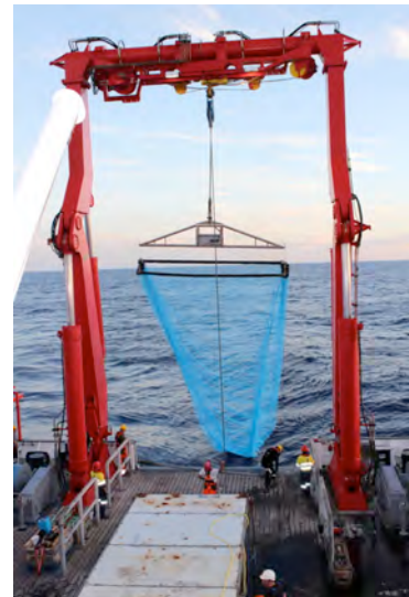
Tucker trawl deployment. (Photo: Nina Furchheim)
