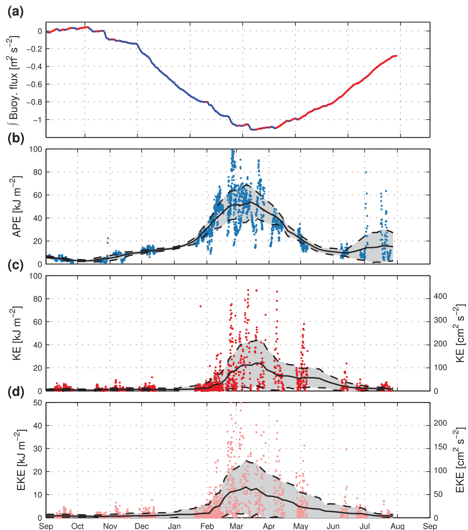
Figure 5. Time series of: (a) integrated buoyancy flux estimated at the LION meteorological buoy (blue dots indicate negative net heat flux, and red positive ones); (b) Available Potential Energy (APE) integrated from the surface down to 1,000 m from all glider density profiles; (c) total Kinetic Energy (KE); and (d) Eddy Kinetic Energy (EKE) estimated for 0–1,000 m layer from the glider depth-average currents. The black line shows the mean signal binned into 5 days period and smoothed with a moving average of 30 days. The gray-shaded area represents the standard deviation in each 5 days bin.
