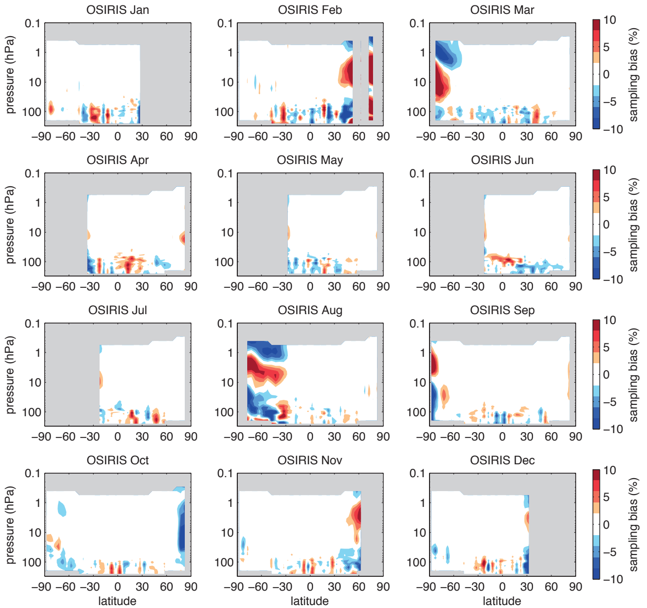
Figure A3.1.7: Sampling error for OSIRIS. Latitude-height sections of calculated sampling error for OSIRIS O_3 for all months. Grey regions denote regions of no measurements.
