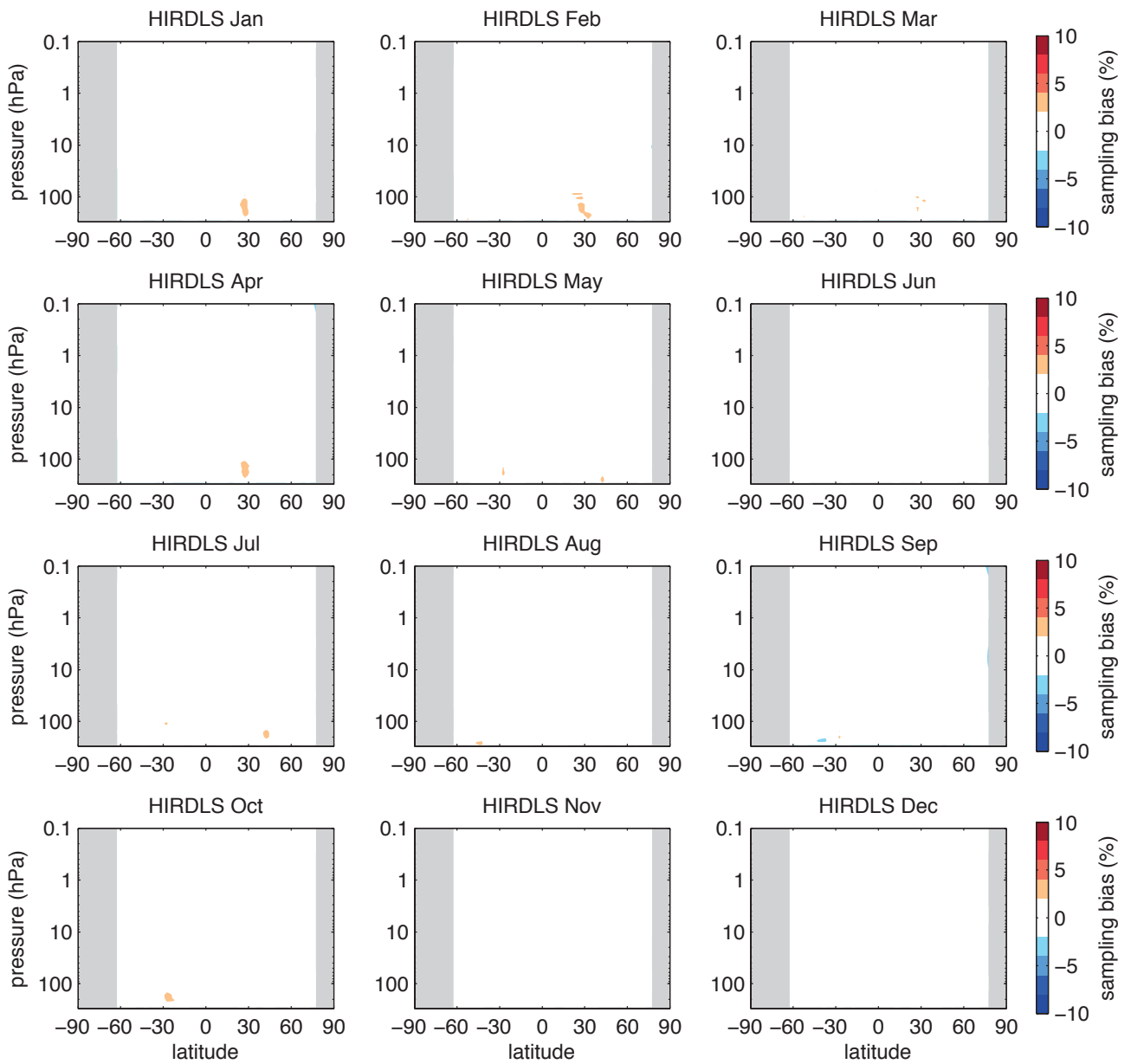
Figure A3.1.5: Sampling error for HIRDLS. Latitude-height sections of calculated sampling error for HIRDLS O_3 for all months. Grey regions denote regions of no measurements.
