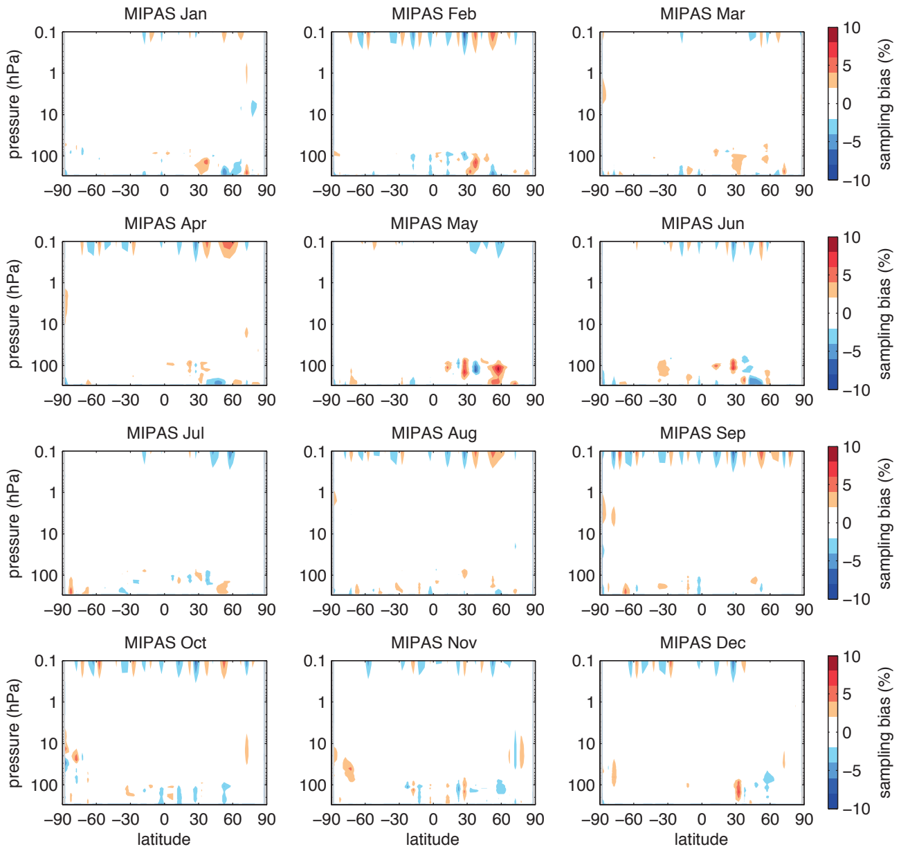
Figure A3.1.6: Sampling error for MIPAS. Latitude-height sections of calculated sampling error for MIPAS O_3 for all months. Grey regions denote regions of no measurements.
