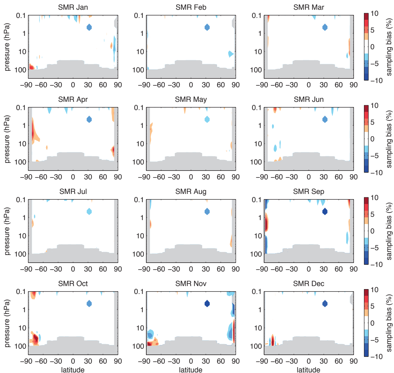
Figure A3.1.14: Sampling error for SMR. Latitude-height sections of calculated sampling error for SMR O 3 for all months. Grey regions denote regions of no measurements.
