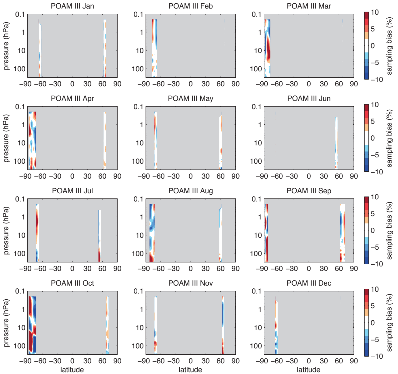
Figure A3.1.9: Sampling error for POAM III. Latitude-height sections of calculated sampling error for POAM III O 3 for all months. Grey regions denote regions of no measurements.
