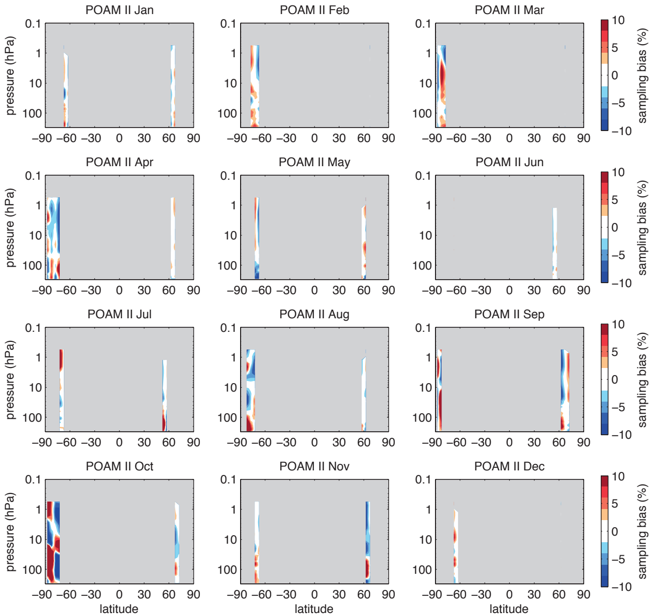
Figure A3.1.8: Sampling error for POAM II. Latitude-height sections of calculated sampling error for POAM II O 3 for all months. Grey regions denote regions of no measurements.
