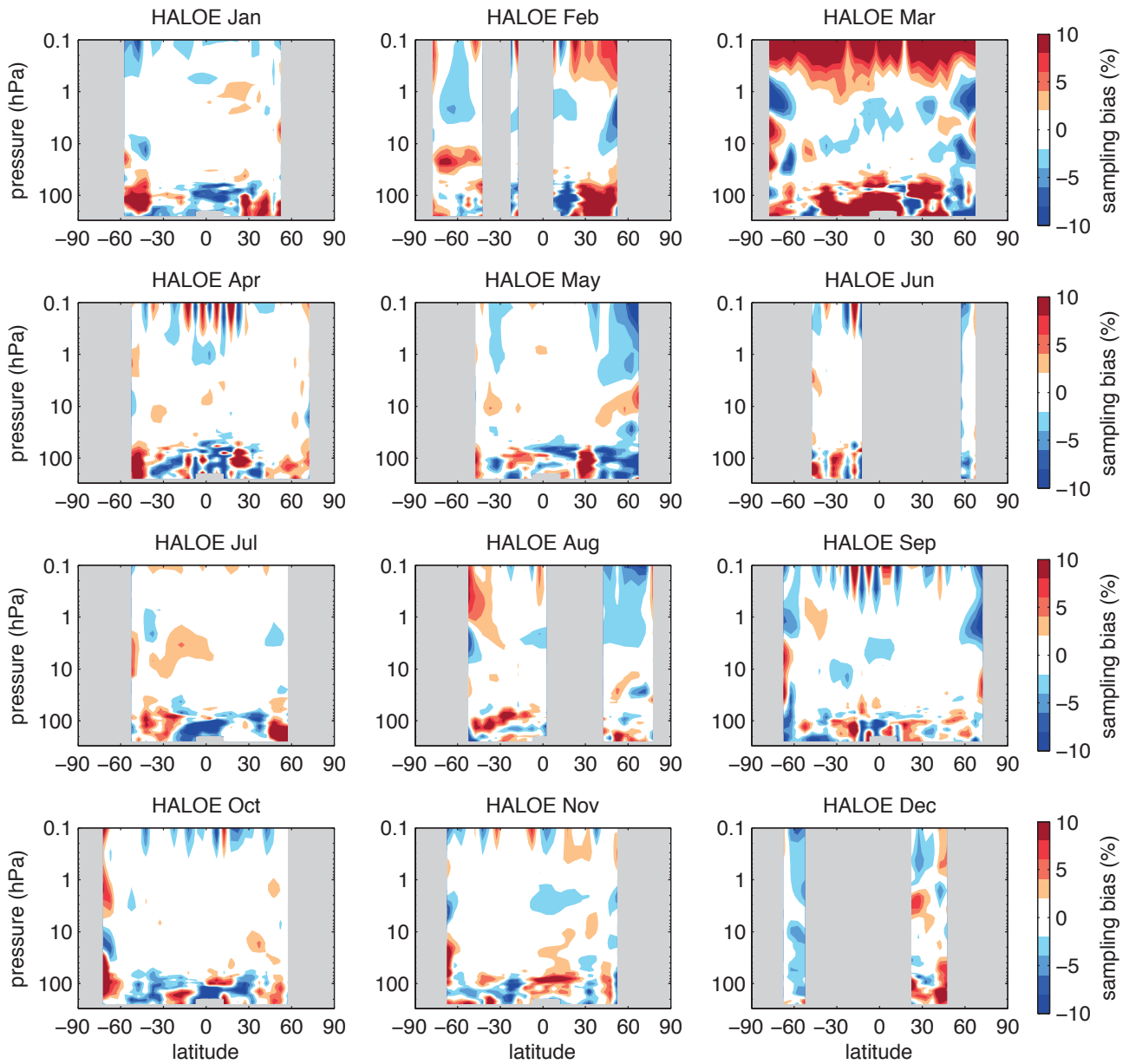
Figure A3.1.4: Sampling error for HALOE. Latitude-height sections of calculated sampling error for HALOE O_3 for all months. Grey regions denote regions of no measurements.
