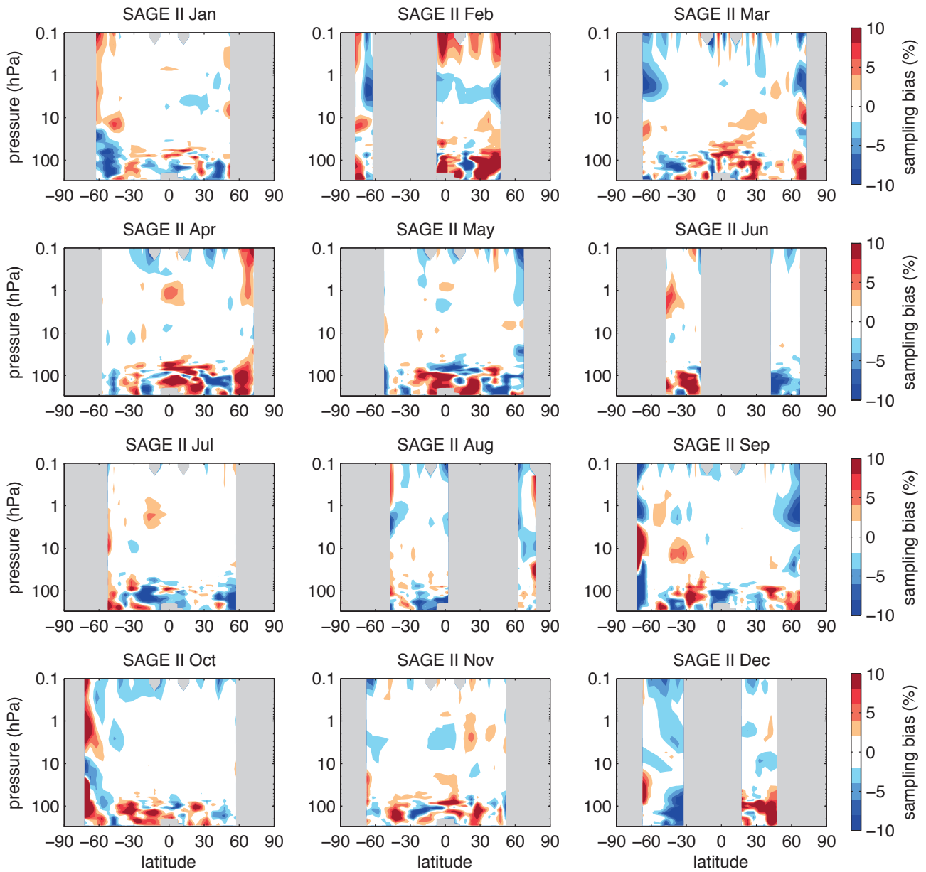
Figure A3.1.10: Sampling error for SAGE II. Latitude-height sections of calculated sampling error for SAGE II O_3 for all months. Grey regions denote regions of no measurements.
