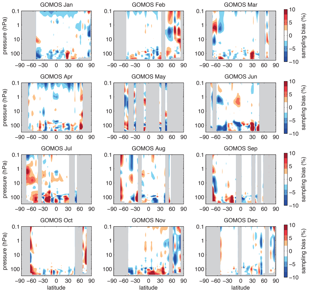
Figure A3.1.3: Sampling error for GOMOS. Latitude-height sections of calculated sampling error for GOMOS O_3 for all months. Grey regions denote regions of no measurements.
