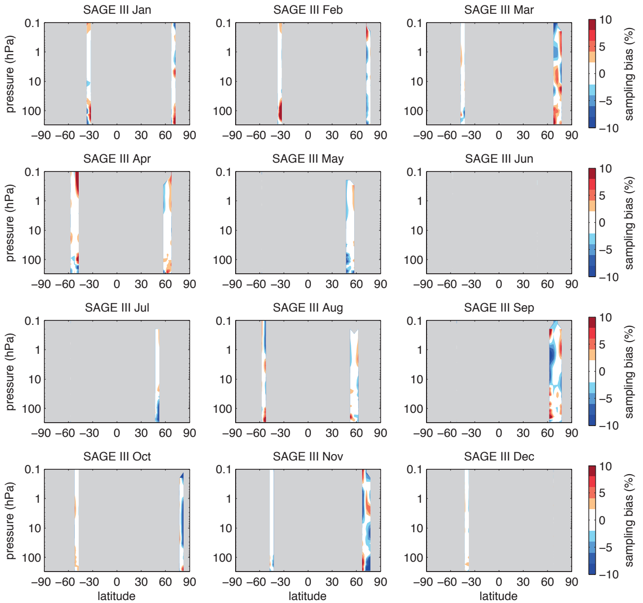
Figure A3.1.11: Sampling error for SAGE III. Latitude-height sections of calculated sampling error for SAGE III O_3 for all months. Grey regions denote regions of no measurements.
