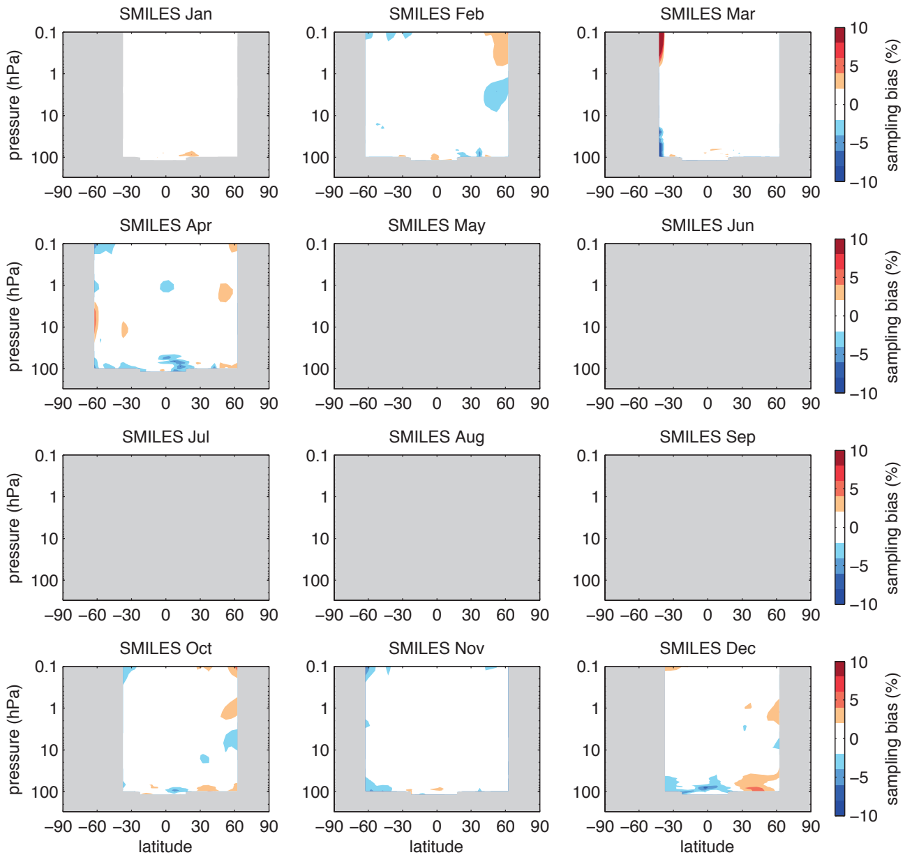
Figure A3.1.13: Sampling error for SMILES. Latitude-height sections of calculated sampling error for SMILES O 3 for all months. Grey regions denote regions of no measurements.
