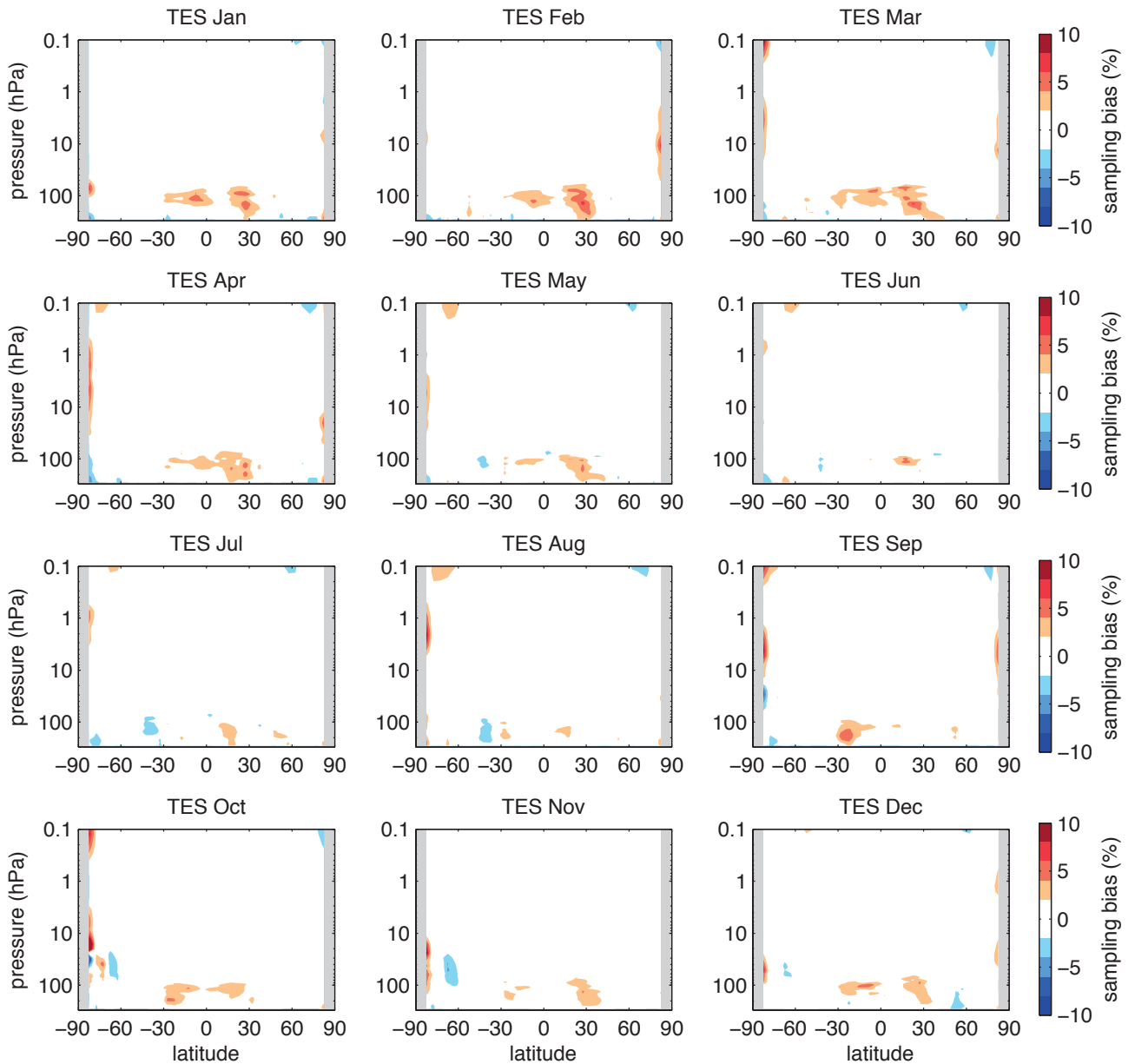
Figure A3.1.15: Sampling error for TES. Latitude-height sections of calculated sampling error for TES O_3 for all months. Grey regions denote regions of no measurements.
