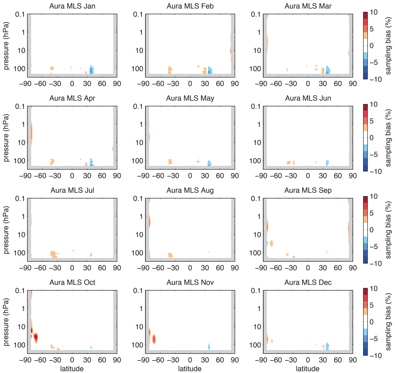
Figure A3.1.2: Sampling error for Aura-MLS. Latitude-height sections of calculated sampling error for Aura-MLS O 3 for all months. Grey regions denote regions of no measurements.
