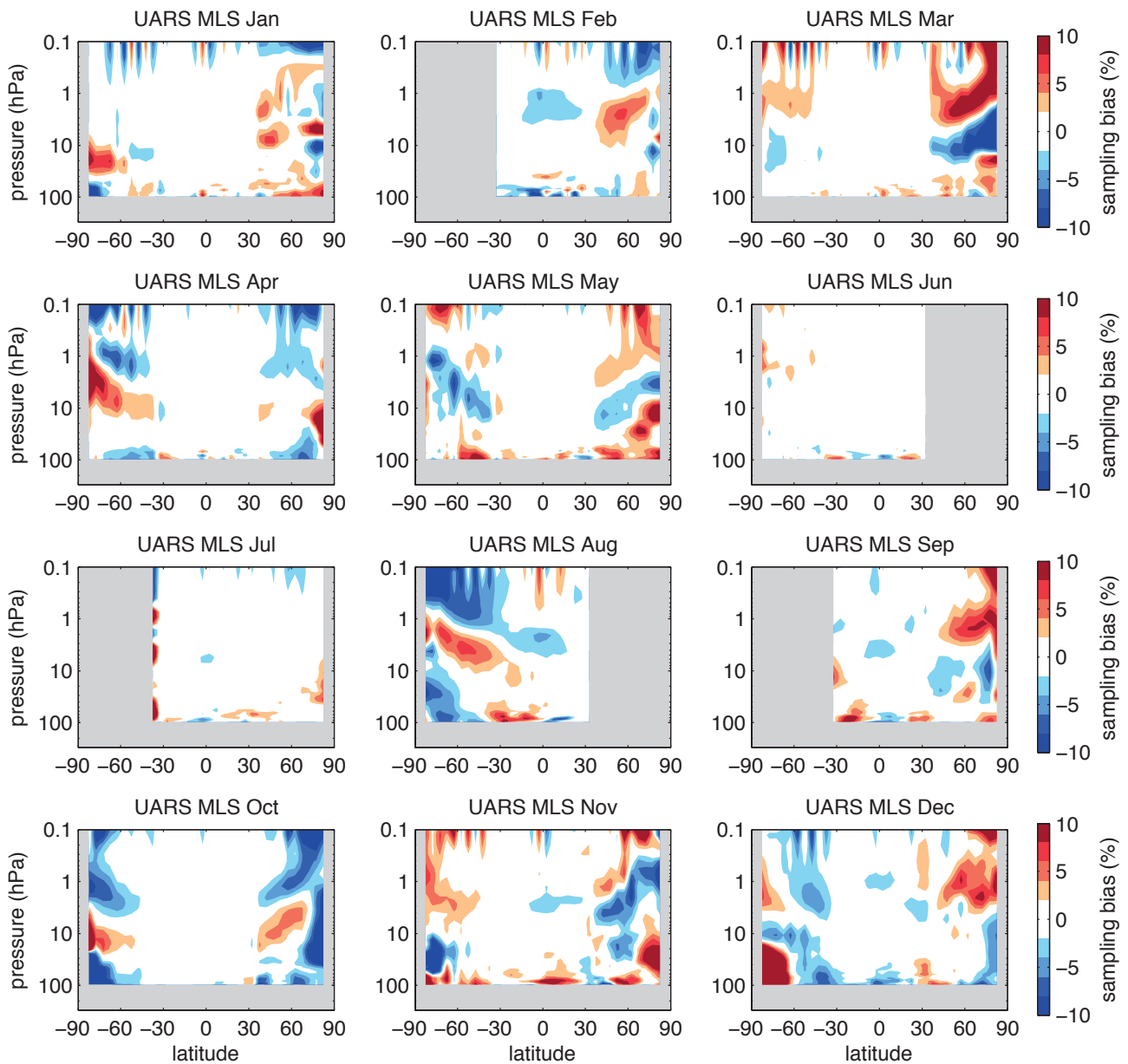
Figure A3.1.16: Sampling error for UARS-MLS. Latitude-height sections of calculated sampling error for UARS-MLS O_3 for all months. Grey regions denote regions of no measurements.
