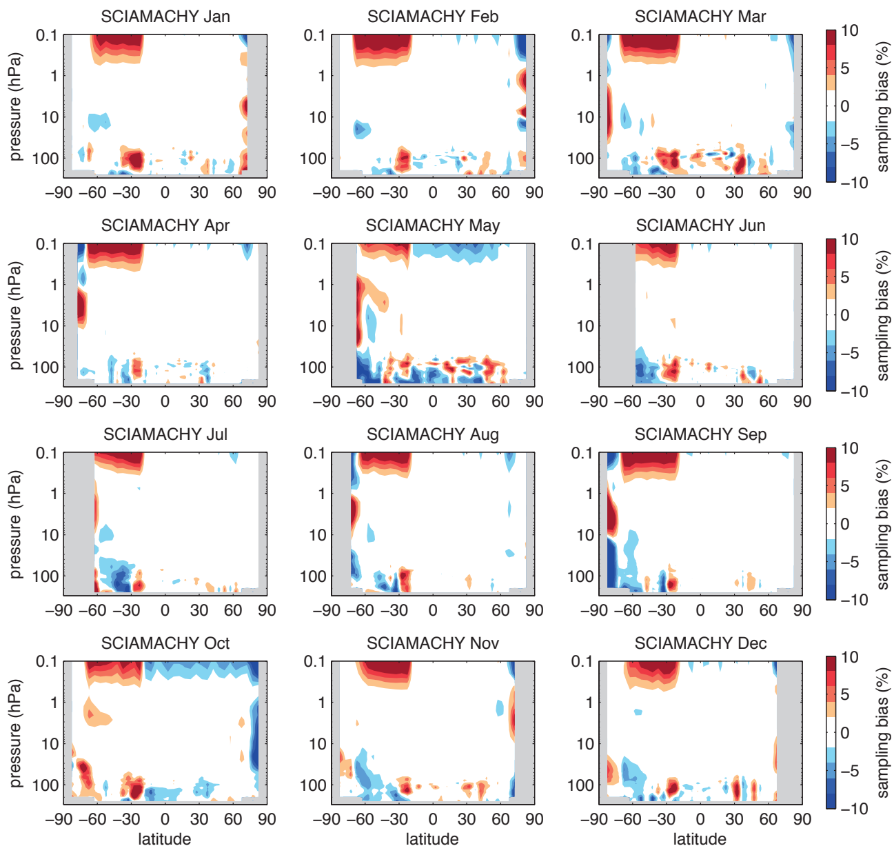
Figure A3.1.12: Sampling error for SCIAMACHY. Latitude-height sections of calculated sampling error for SCIAMACHY O 3 for all months. Grey regions denote regions of no measurements.
