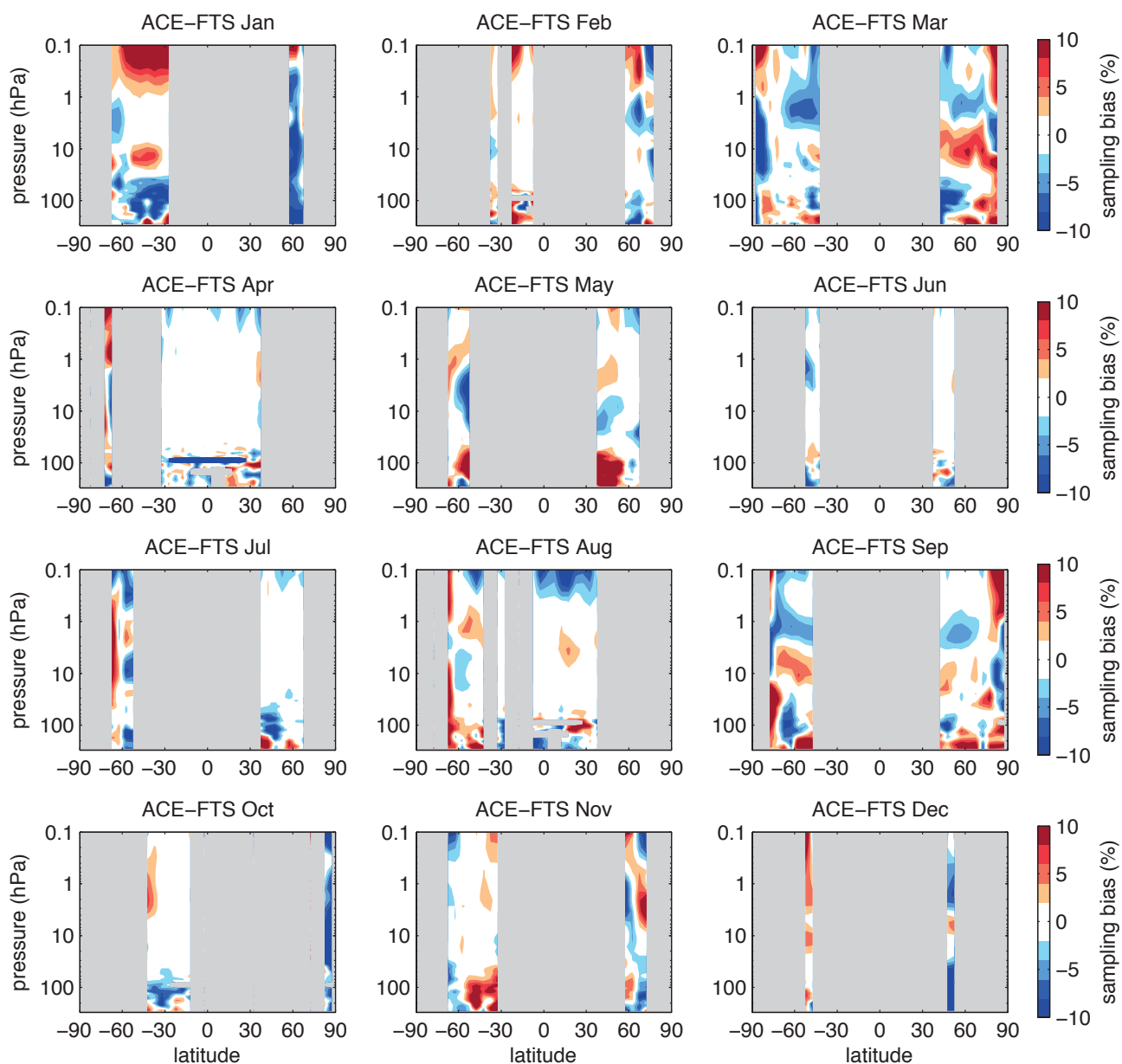
Figure A3.1.1: Sampling error for ACE-FTS. Latitude-height sections of calculated sampling error for ACE-FTS O_3 for all months. Grey regions denote regions of no measurements.
