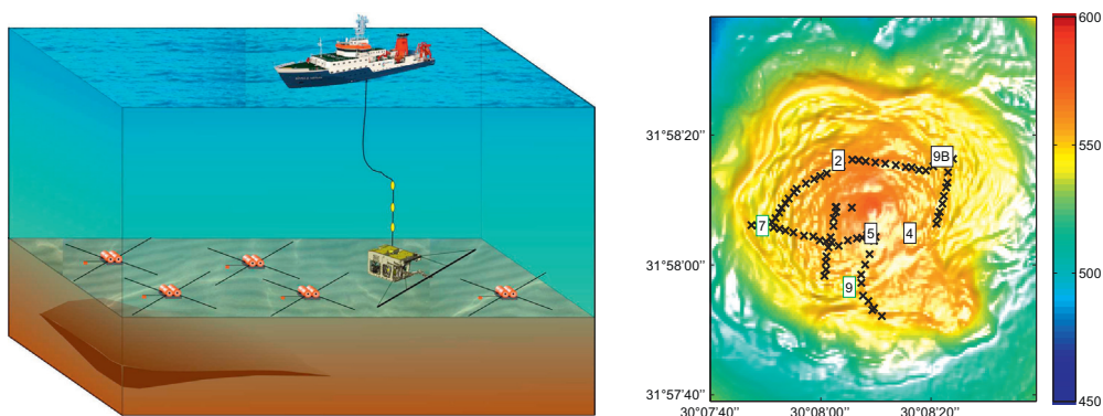
Fig. 8. Left: Design of marine CSEM-system from GEOMAR. A source field is emitted from a dipole antenna, which is mounted on an ROV. The induced secondary fields depend on the spatial conductivity distribution of the subsurface. Horizontal field components are measured at a number of receivers that are deployed at the seafloor. Right: Station map of CSEM-experiment at mud volcano offshore Egypt (Hölz and Jegen, 2009). Crosses and boxes show transmitters and receivers positions, respectively.
