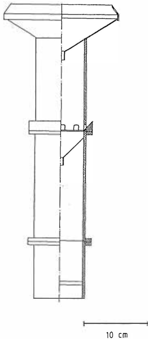
Figure 1: Sketch of mechanical raingauge. Left half is the view from the side, right half shows the cut. The instrument has a cylindrical cross section (80 mm diameter). The horizontal orifice at the top is taken from a standard weather service type Hellmann raingauge of 200 cm 2 size. The vertical collecting surface consists essentially of the cylinder (125 mm height) above the rime. The water amount intercepted by both surfaces is collected each by a cone and fed to a gauging unit in the lower part (not shown here). Counts are recorded either with a PC or with a data logging unit.
