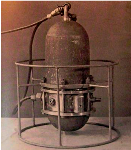
Fig. 9. The first electronic CTD probe for the in-situ observation of vertical temperature and salinity profiles in the upper ocean (Plate 24 in Hinkelmann, 1956). In the protective cage the one-conductor cable with oil filled connector, the pressure inlet, an electrode conductivity cell, and the platinum thermometer are shown from left to right. The upper housing was packed with dozens of thermionic valves.
