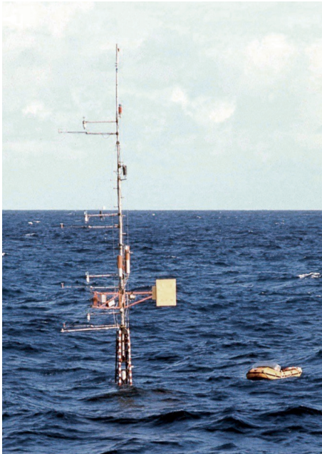
Fig. 22. Meteorological stabilized buoy with sensor packages in the tropical Atlantic Ocean during GATE, 1974. (Photo: H. Skade)
