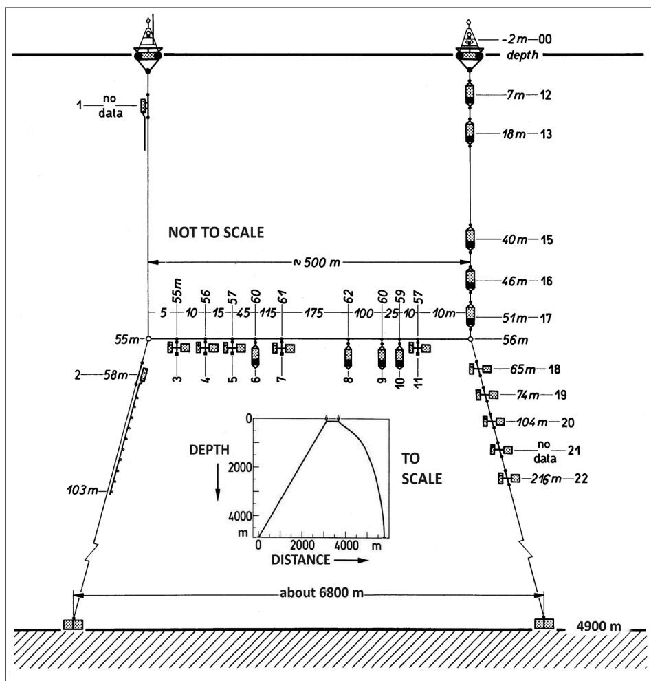
Fig. 18. Design of the GATE mooring F1 for studying internal wave kinematics with the cable configuration for a hypothetical current from left to right (not to scale). In the inner sub-frame the whole construction is shown to scale. (After Käse, Siedler, 1980)
